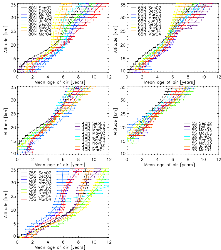
Fig. 10. Monthly zonal mean age of stratospheric air profiles for 80° N, 65° N, 40° N, 5° S, and 75° S for the months September 2002 (black), December 2002 (violet), March 2003 (dark blue), May 2003 (light blue), June 2003 (turquoise), September 2003 (green), November 2003 (yellow), January 2004 (orange), and March 2004 (red). Errors represent the 1\sigma standard errors of the mean (horizontal lines).
