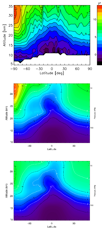
Fig. 13. Zonal mean distribution of mean age of stratospheric air for October 2003 from MIPAS (top), and KASIMA with (middle) and without (bottom) consideration of the SF 6 loss reaction in the mesosphere, giving the apparent and the true mean age, respectively.
