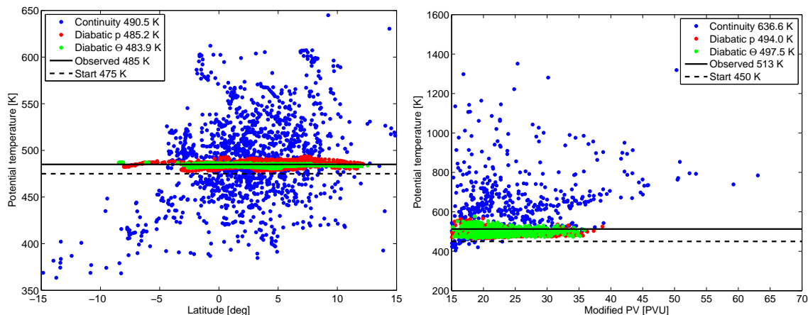
Fig. 2. Trajectory runs driven with different vertical wind fields. Left: Position of 1440 forward trajectories started at 1 January 2000 (00 h UTC) on the equator after 20 days, for winds from the continuity equation in pressure coordinates (blue dots), from the thermodynamic equation in pressure coordinates (red dots) and from heating rates in \theta coordinates (green dots). Right: Position of backward trajectories on 26 November 1999 (12 h UTC) started at 450 K inside the polar vortex on a 2.5^\circ grid on 5 March 2000 (12 h UTC).
