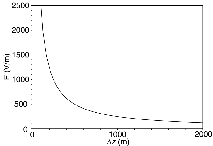
Fig. 6. Electric field gradient as a function of aerosol layer thickness for optical depth of 0.31, calculated from Eq. (12) with the topographic enhancement factor of two.
