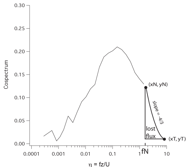
Fig. 2. Archetype of an observed cospectrum, showing the showing the terminal observed value of the cospectrum well above zero at the normalized Nyquist frequency ( fN ). Extending a line from this point to zero using a -4/3 slope shows an area of the flux in the inertial subrange that is unresolved by the measurement frequency, and is called here the “lost flux”. That the plotted points of the cospectrum represent midpoints of bins in the observed cospectrum, so the terminal bin is bounded by fN on the high frequency end. Note that this graph is semilog, making the -4/3 slope non linear.
