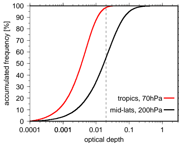
Fig. 5. Frequency distribution of the contrail optical depth as simulated by ECHAM4 for the 2050 mixed fleet scenario S5 and for different geographical regions. Red: tropical lower stratosphere ( 20^{\circ} N– 20^{\circ} S, 70 hPa), black: northern extratropical upper troposphere ( 70^{\circ} N– 40^{\circ} N, 200 hPa). The threshold optical depth of 0.02 is indicated by the vertical dashed line.
