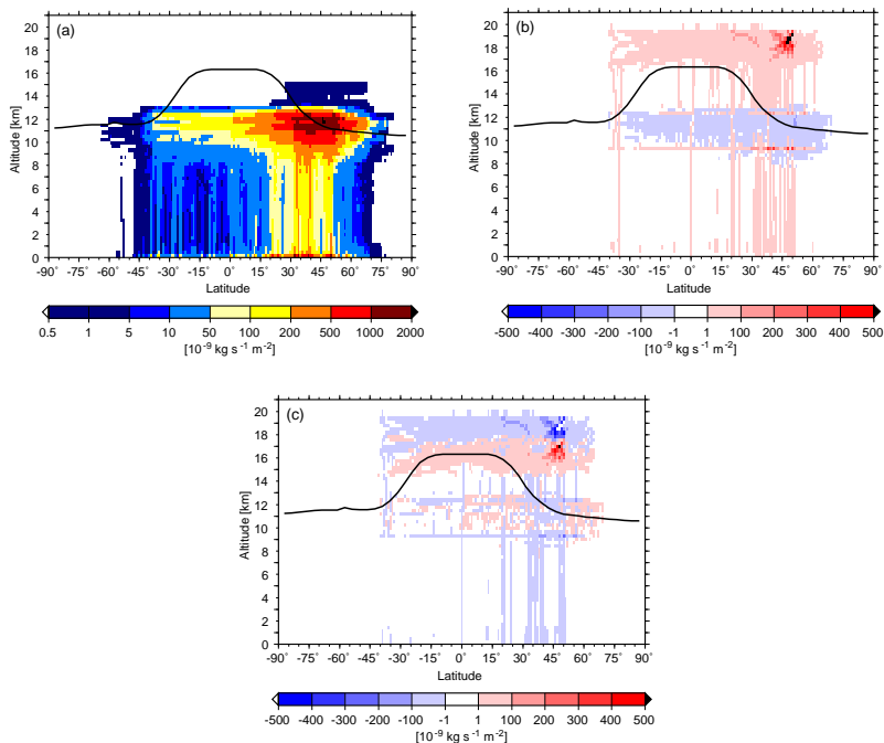
Fig. 1. Horizontally integrated fuel consumption [10^{-9} \text{ kg s}^{-1} \text{ m}^{-2}] of commercial aircraft considered in the SCENIC subsonic fleet for 2050 (a) . Difference between the 2050 mixed and subsonic fleet S5-S4 (b) and between the mixed fleet scenarios P4-S5 (c) . The black line indicates a zonal and annual mean tropopause height.
