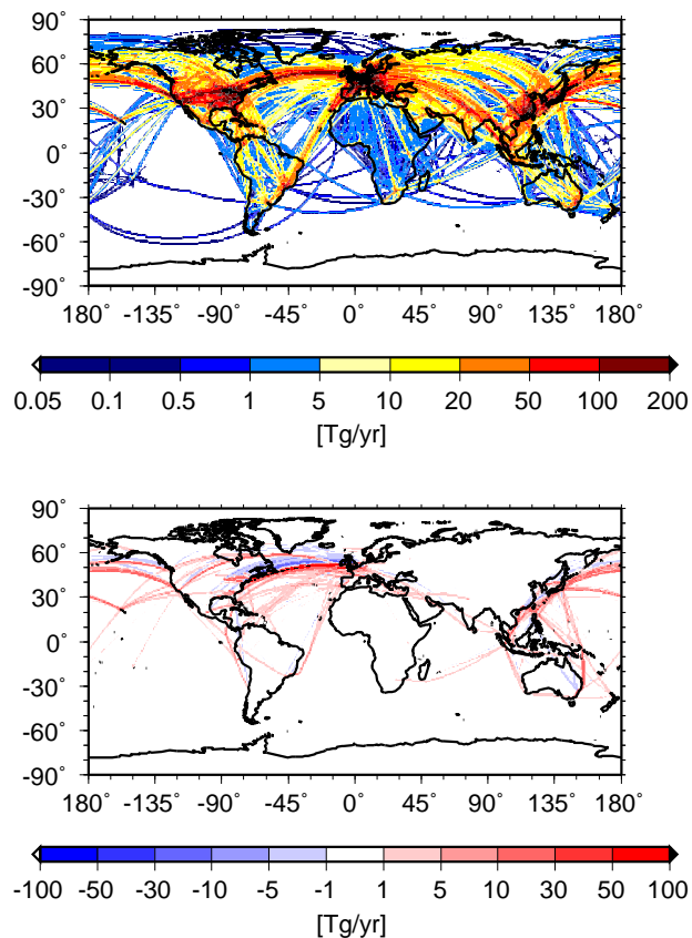
Fig. 2. Upper panel: Horizontal distribution of the vertically integrated fuel consumption of commercial aircraft considered in the SCENIC subsonic fleet for 2050 (S4) [Tg yr -1 ]. Lower panel: Difference between the 2050 mixed and subsonic fleet S5-S4 [Tg yr -1 ].
