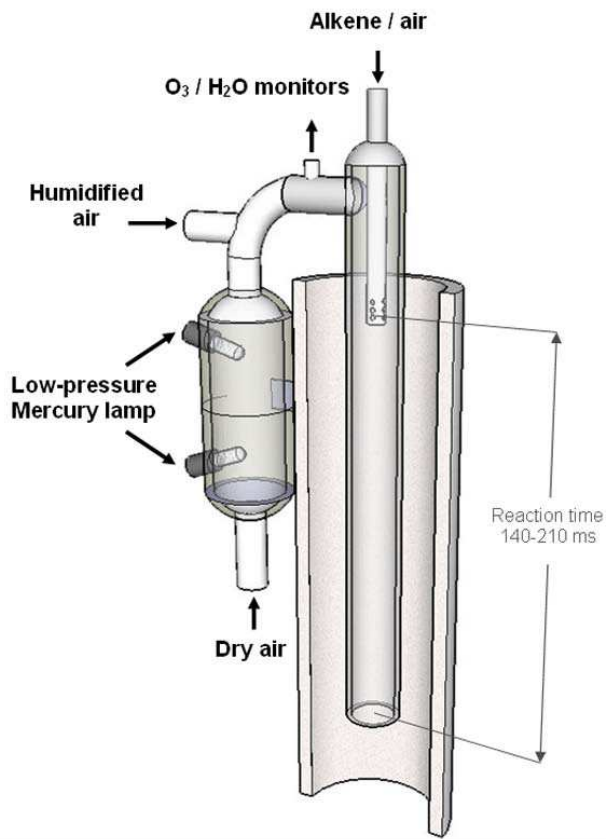
Fig. 4. Schematic of the calibrator based on the steady-state O 3 -alkene technique.
