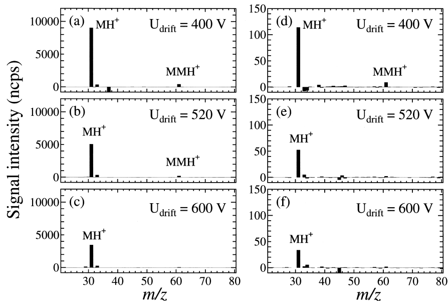
Fig. 2. Mass spectrum of HCHO at three different drift tube E/N ratios, obtained by the direct introduction method (a–c) and dynamic dilution method (d–f). (a–c): [\text{HCHO}] = 1.02 ppmv; (d–f): [\text{HCHO}] = 23.3 ppbv. Signals were normalized to a \text{H}_3\text{O}^+ intensity of 10^6 cps.
