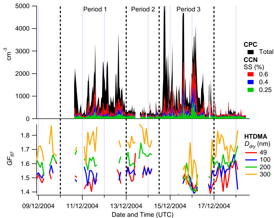
Fig. 3. CCN number concentrations and mean HTDMA growth factors measured at the Cape San Juan site.
