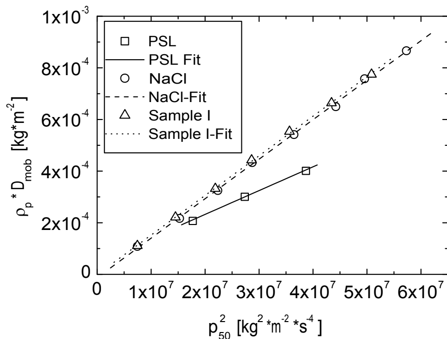
Fig. A2. The product \rho_p D_{\text{mob}} is plotted against p_{50}^2 for the PSL, NaCl and sea-salt (sample I) particles, to determine the shape factor of the different sea-salt particles.
