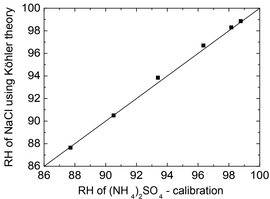
Fig. 2. RHs as determined from the hygroscopic growth of NaCl particles with D_{me_0} = 189 nm are plotted versus RHs resulting from the calibration with ammonium sulfate particles with D_{me_0} = 200 nm.
