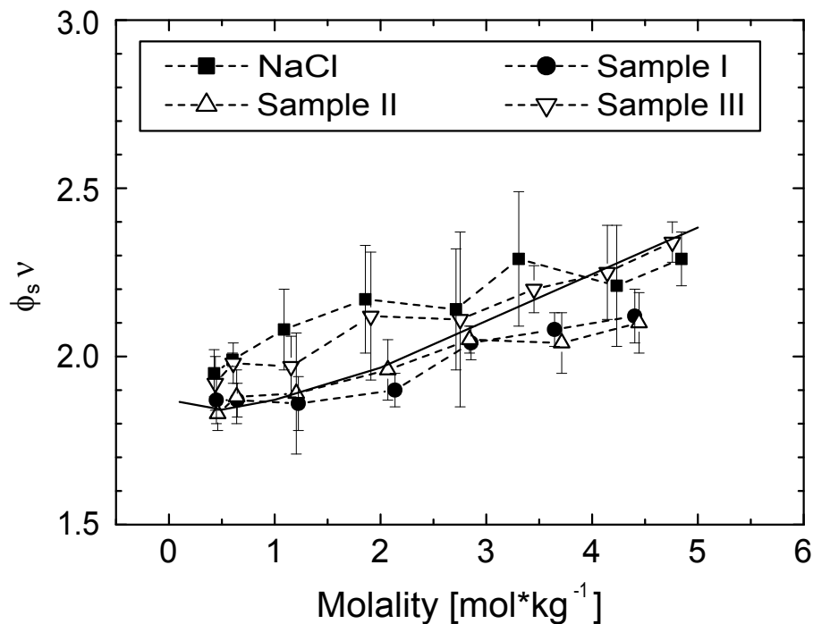
Fig. 7. \phi_{s,v} derived from the measured hygroscopic growth for NaCl and the three sea-salt samples in comparison to values for NaCl as given in literature (Pruppacher and Klett, 1997).
