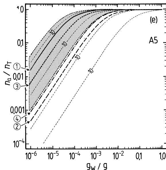
Fig. 5. Fractions of the water-soluble semi-volatile surrogate compounds A1 to A2 present in the aerosol phase at 298.15 K, calculated using Eq. (2a) for different estimates of p_i^{\circ} , and plotted against atmospheric liquid water content g_w ( \text{g m}^{-3} ). Unit activity coefficients are assumed. The thin dashed lines represent the calculated partitioning at intervals of factors of 10 in f_i p_i^{\circ} . Vapour pressure estimates, Table 6, were obtained using the equation of Myrdal and Yalkowsky (1997) together with boiling points estimated by the following methods: 1 – value used in UCD-CACM model, without adjustment (solid line); 2 – Nannoolal et al. (2004) (dashed line); 3 – ACD software (dotted line); 4 – a direct prediction of vapour pressure using the method of Asher (Asher and Pankow, 2006; Asher et al., 2002) (dash-dot line). The shaded area corresponds to vapour pressures calculated using the ACD boiling point, plus/minus its estimated uncertainty which is listed in Table 3. (a) Surrogate compound A1; (b) A2; (c) A3; (d) A4; (e) A5.
