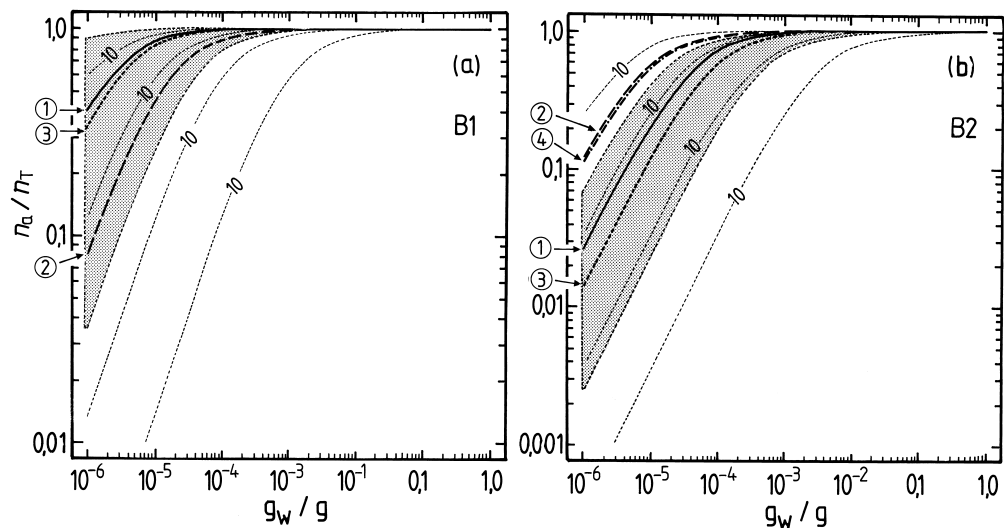
Fig. 4. Fractions of the water-soluble semi-volatile surrogate compounds B1 and B2 present in the aerosol phase at 298.15 K, calculated using Eq. (2a) for different estimates of p_i^{\circ} , and plotted against atmospheric liquid water content g_w ( \text{g m}^{-3} ). Unit activity coefficients are assumed. The thin dashed lines represent the calculated partitioning at intervals of factors of 10 in f_i p_i^{\circ} . Vapour pressure estimates, Table 7, were obtained using the equation of Myrdal and Yalkowsky (1997) together with boiling points estimated by the following methods: 1 – value used in UCD-CACM model, without adjustment (solid line); 2 – Nannoolal et al. (2004) (dashed line); 3 – ACD software (dotted line); 4 – a direct prediction of vapour pressure using the method of Asher (Asher and Pankow, 2006; Asher et al., 2002) (dash-dot line). The shaded area corresponds to vapour pressures calculated using the ACD boiling point, plus/minus its estimated uncertainty which is listed in Table 3. (a) Surrogate compound B1; (b) surrogate compound B2.
