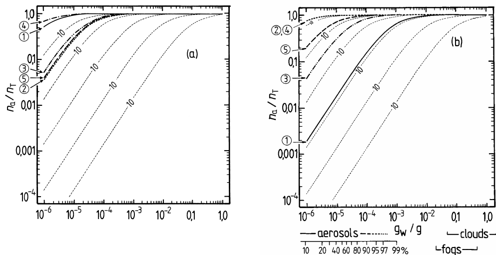
Fig. 3. Fractions of the semi-volatile surrogate compounds present in the aerosol phase, calculated using Eq. (2a), plotted against atmospheric liquid water content ( g_w/g\text{ m}^{-3} ) for T=298.15\text{ K} . Solubility in water and unit activity coefficients are assumed, and the values of p_i^\circ are those used in the UCD-CACM model, including the downward adjustments to account for the effects of chemical reactions. The thin dashed lines represent the calculated partitioning at intervals of factors of 10 in f_i p_i^\circ . (a) Lines – surrogate species B1-5, indicated by the circled numbers on the y-axis; (b) lines – surrogate species A1-5. Approximate ranges of atmospheric liquid water content associated with clouds, fogs and aerosols (including typical RH based on 10^{-4}\text{ g m}^{-3} of aerosol water at 90% RH, and an acid ammonium sulphate aerosol) are indicated.
