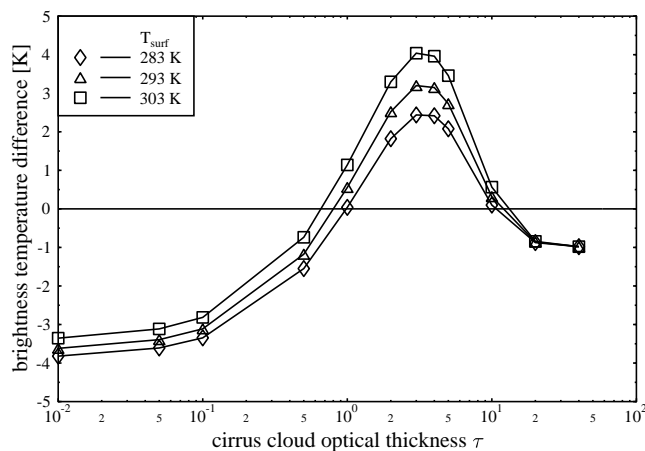
Fig. 7. Simulated brightness temperature difference T_{8.7} - T_{10.8} between SEVIRI infrared channels IR8.7 and IR10.8 for the mid-latitude summer atmosphere, a cirrus cloud between 10 and 11 km, effective particle radius 6 \mu\text{m} , and satellite zenith angle 60^\circ , as a function of optical thickness \tau for three different surface temperatures.
