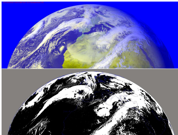
Fig. 11. (Top) False color composite MSG image for 3 March 2004, 14:30 UTC; (bottom) corresponding MeCiDA cirrus mask.
