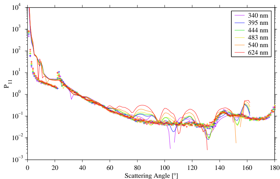
Fig. 5. Measured (solid lines) and theoretical (+'s) phase functions for mixed cloud 03.
