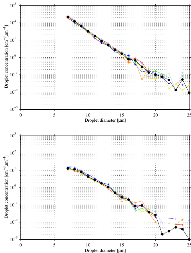
Fig. 2. 2 PSDs for water clouds 14 & 17 at 2 min intervals (blue through red; black is mean).
