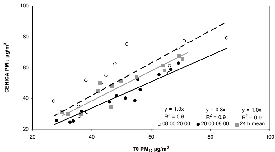
Fig. 2. Comparison of 12 and 24 h PM 10 levels simultaneously measured at T0 and CENICA (two urban background sites), Mexico City, during the MILAGRO campaign.
