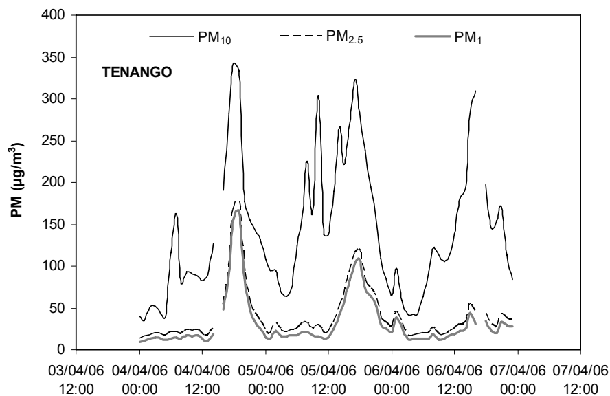
Fig. 5. Hourly PM levels measured at the rural site Tenango, showing the Mexico City's plume impact causing high levels of \text{PM}_1 .
