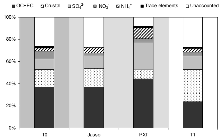
Fig. 9. Mean PM_{10} (top) and PM_{2.5} (bottom) composition obtained at urban (grey dark), industrial-rural (grey clear) and suburban and rural rural sites.
