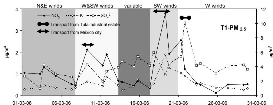
Fig. 11. 12 h levels (daylight and night) of nitrate, potassium and sulfate in PM 2.5 measured at the T1 suburban site on 1, 3, 5, 7, 9, 11, 13, 16, 17, 19, 21, 23, 25, 27 and 29 March 2006. Note that nitrate and potassium trace the transport from México City, whereas sulfate is mainly tracing the transport from Tula industrial estate. The transport and synoptic scenarios described by Fast et al. (2007) for the MILAGRO campaign are also marked in the plot.
