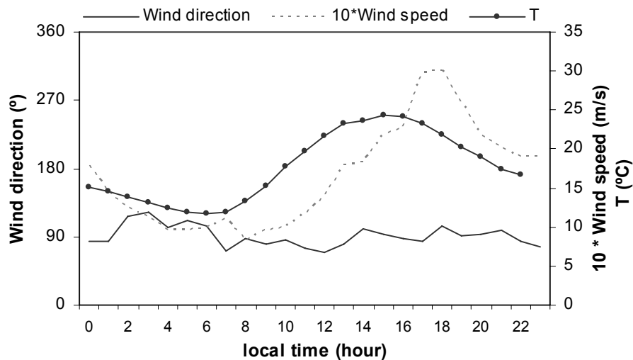
Fig. 4. Mean hourly temperature, wind direction and wind speed recorded at T0 from 1 to 26 March 2006.
