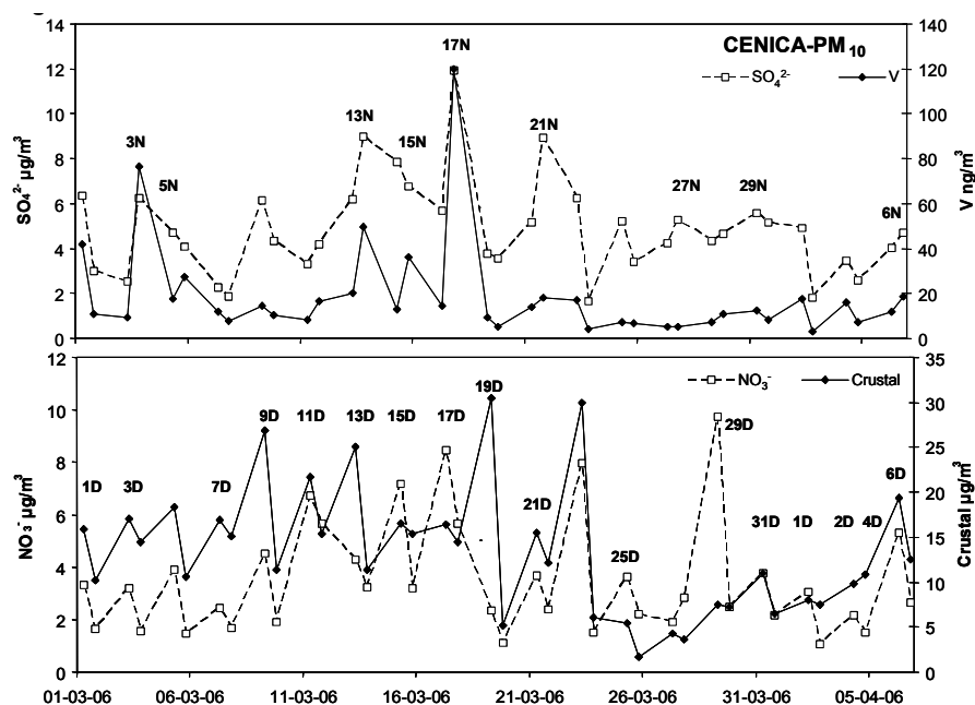
Fig. 7. Mean 12 h levels of \text{SO}_4^{2-} , \text{NO}_3^- , V and crustal material recorded at CENICA during the MILAGRO campaign. N, maximum value recorded in the nighttime sample; D maximum value recorded in the daylight sample.
