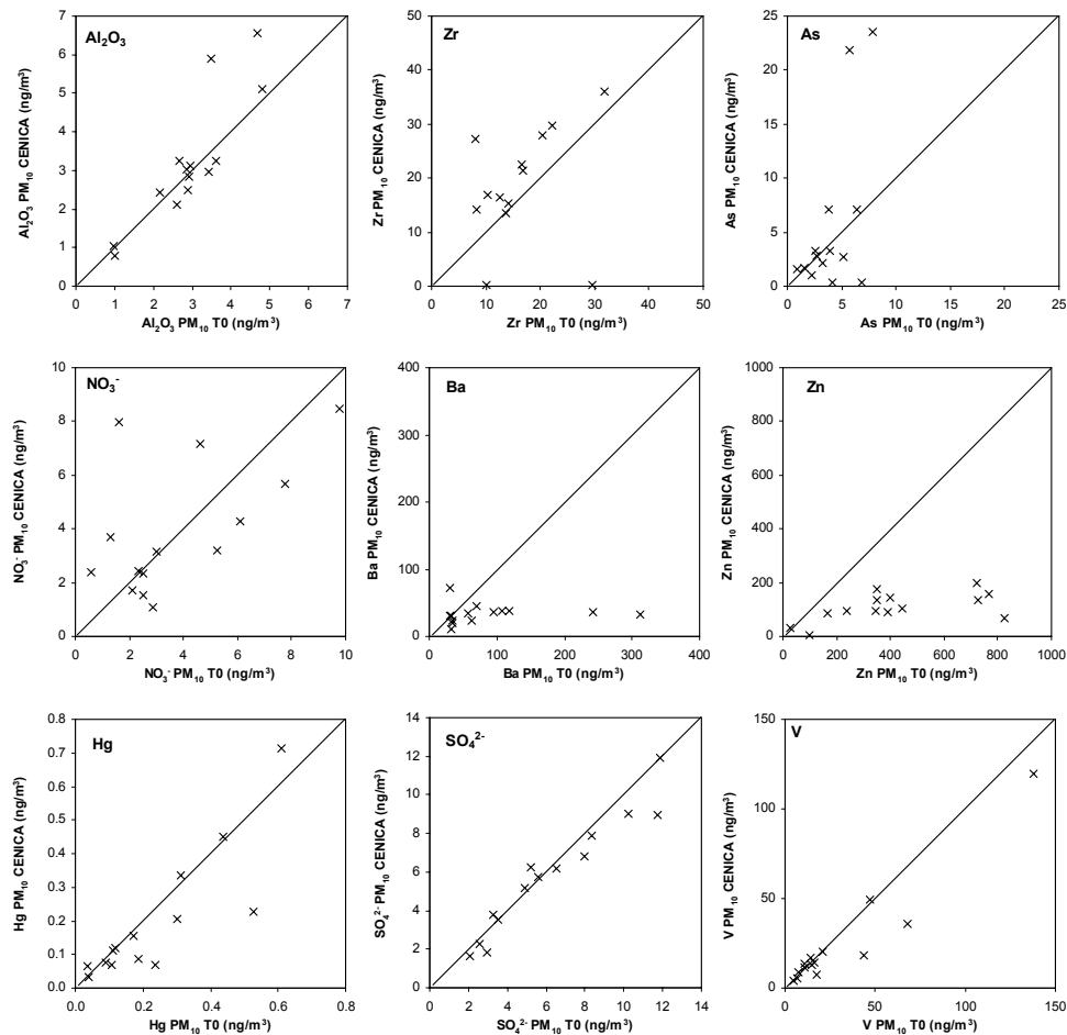
Fig. 8. Correlation between levels of \text{Al}_2\text{O}_3 , Zr, As, \text{NO}_3^- , Ba, Zn, Hg, V and \text{SO}_4^{2-} in \text{PM}_{10} at CENICA and T0.
