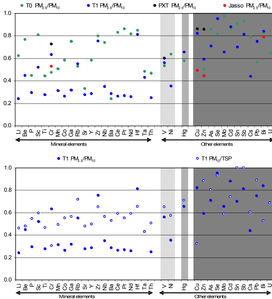
Fig. 10. PM_{2.5}/PM_{10} ratios of trace elements levels at T0, T1, Jasso and PXT. PM_{10}/TSP levels at T1.
