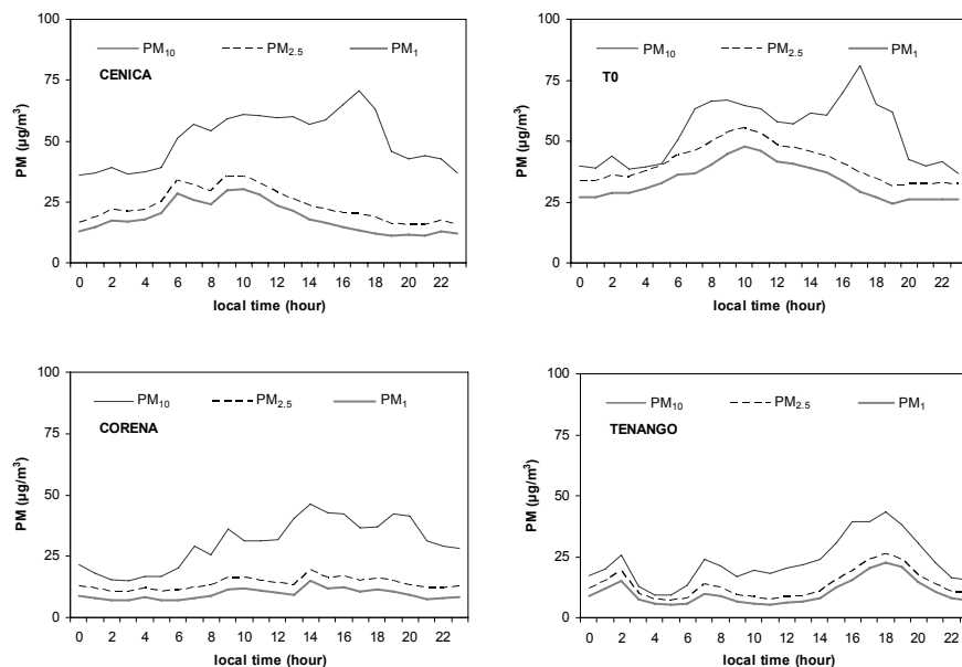
Fig. 3. Mean hourly PM levels measured during the whole MILAGRO campaign at 2 urban background sites of Mexico City, CENICA and T0, and at two southern sites, Tenango and Corena.
