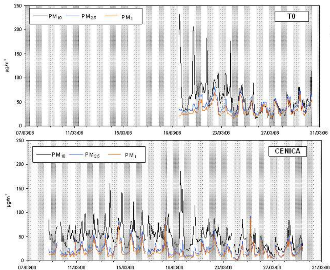
Fig. 6. Hourly PM levels measured during the whole MILAGRO campaign at 2 urban background sites of Mexico City, CENICA and T0.
