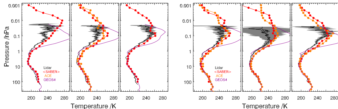
Fig. 7. Lidar profiles taken at Eureka on selected days in February and March 2004 compared with coincident profiles from SABER (red lines with dots), ACE (orange lines with dots), and GEOS-4 (purple lines without symbols). Lidar profile is in black, with 1- \sigma uncertainty range shown as grey shading.
