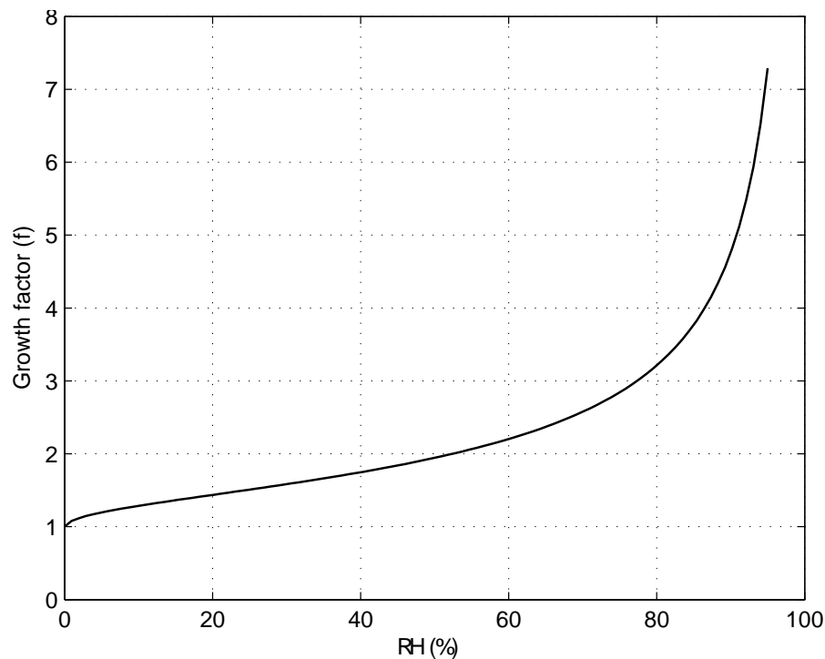
Fig. 3. Growth factor (growth factor(f) = \frac{m_{\text{H}_2\text{SO}_4} + m_{\text{H}_2\text{O}}}{m_{\text{H}_2\text{SO}_4}} ) of sulfate-water particle with respect to RH (%). The data is obtained from Jaeger-Voirol et al. (1990).
