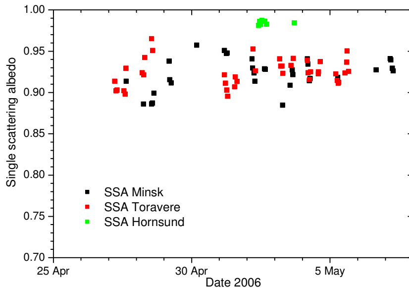
Fig. 6. Column single scattering albedo retrieved from Cimel photometer data at Hornsund, Toravere and Minsk.
