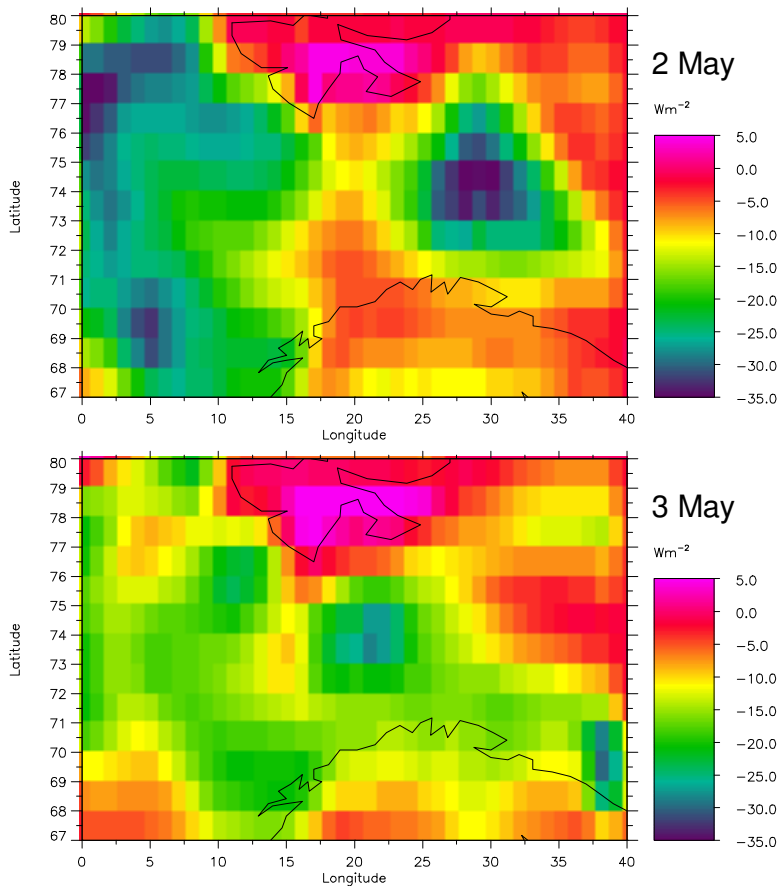
Fig. 9. Radiative forcing of the episode relative to an aerosol situation in the spring with AOD=0.05.
