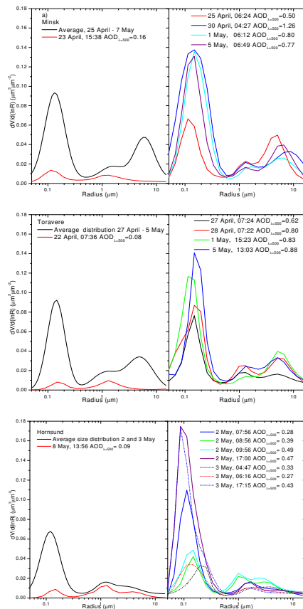
Fig. 5. Volume aerosol size distributions during the smoke transport event: (a) Minsk, (b) Toravere, (c) Hornsund. Right panel: Average distribution of the most intense period together with typical distribution. Right panel: Selected distributions during the period. AOD is given at 500 nm.
