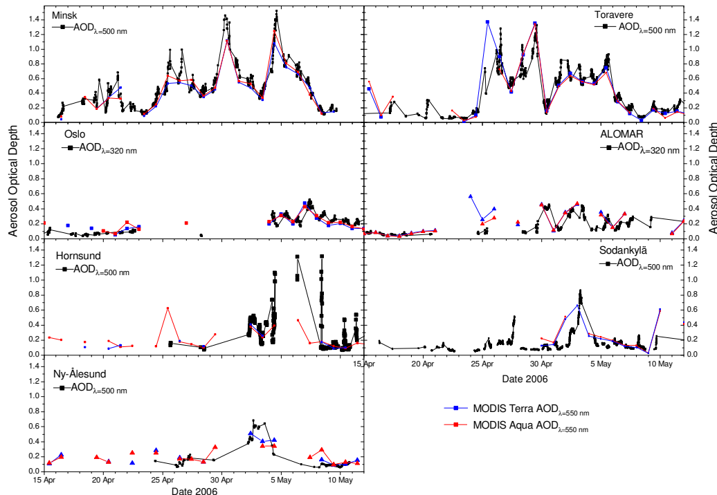
Fig. 7. Comparison of 1^\circ \times 1^\circ grid averaged MODIS AOD and AOD from the ground based stations in the period 15 April–15 May 2006. The MODIS AOD from Aqua and Terra is the red and blue curves respectively in all panels.
