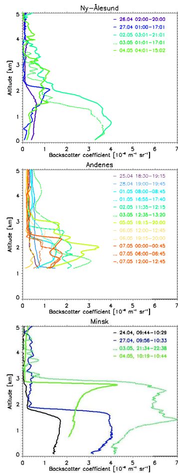
Fig. 8. Height profiles of backscatter coefficients of aerosols from ground based observations at the sites in Ny-Ålesund, Andenes (ALOMAR), and Minsk during spring 2006.
