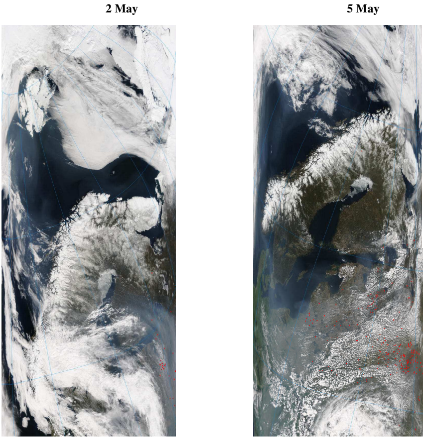
Fig. 2. The plume is clearly seen in the MODIS pictures of northeast Europe and Northern Scandinavia. The red dots in Eastern Europe indicate fires.
