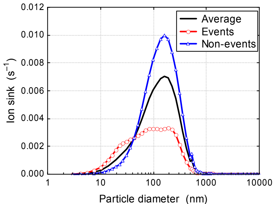
Fig. 2. Ion sink as a function of particle size (factor dN/d\log(d)\cdot w(d) ) for the nucleation event days, non-event days and the average of the period of 31 March–29 April 1999. Hyytiälä station.
