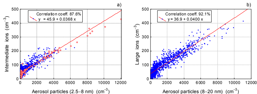
Fig. 5. Scatterplot between the concentrations of positive aerosol ions and aerosol particles: (a) aerosol ions ( m ; 2.5–8 nm), or intermediate ions, versus nanometer aerosol particles (2.5–8 nm). The data points corresponding to 5 April are marked with red squares ( \square ). (b) Aerosol ions ( N ; 8–ca. 20 nm), or large air ions, versus aerosol particles (8–20 nm). Nucleation event days, 31 March–29 April 1999, Hyytiälä station.
