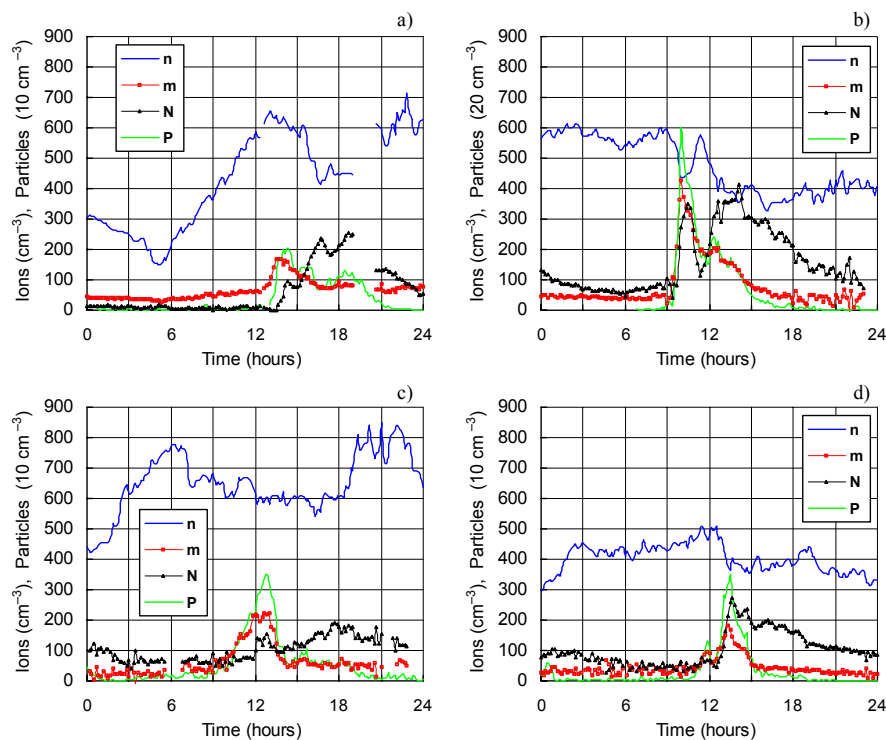
Fig. 6. Diurnal variation in the concentration of positive air ion classes: small ions ( n ; diameters less than 2.5 nm), charged fine nanometer particles ( m ; 2.5–8 nm) and coarse nanometer particles ( N ; 8–ca. 20 nm), as well as the total concentration of particles ( P ; 2.5–8 nm) measured by the DMPS on 2 April (a), 5 April (b), 10 April (c) and 14 April 1999 (d) at Hyytiälä.
