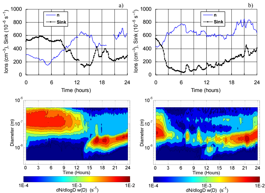
Fig. 7. Diurnal variation in the concentration of positive small ions ( n ), ion sink ( S_a ) and the size distribution of ion sink due to aerosol particles (3–500 nm) on 2 April (a; left) and 10 April 1999 (b; right) at Hyytiälä.
