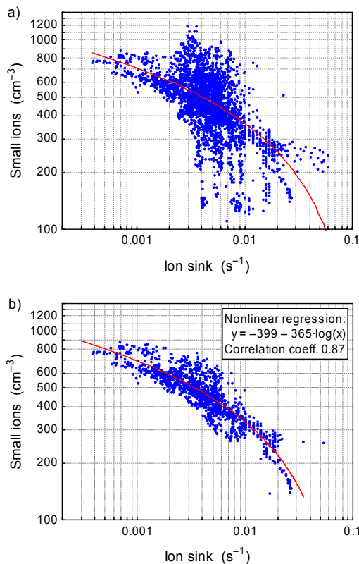
Fig. 3. Scatterplot of the concentration of positive small air ions ( n ) versus ion sink ( S_a ) due to aerosol particles (3–500 nm) and a logarithmic regression line. (a) all the data, (b) selected data when no fog was recorded, relative humidity is less than 95%, and the wind speed is higher than 0.6 \text{ m s}^{-1} . 31 March–29 April 1999, Hyttiälä station.
