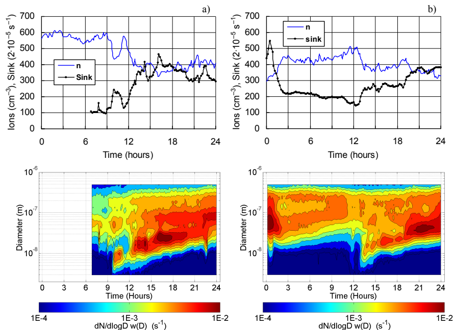
Fig. 8. Diurnal variation in the concentration of positive small ions ( n ), ion sink ( S_a ) and the size distribution of ion sink due to aerosol particles (3–500 nm) on 5 April (a; left) and 14 April 1999 (b; right) at Hyytiälä.
