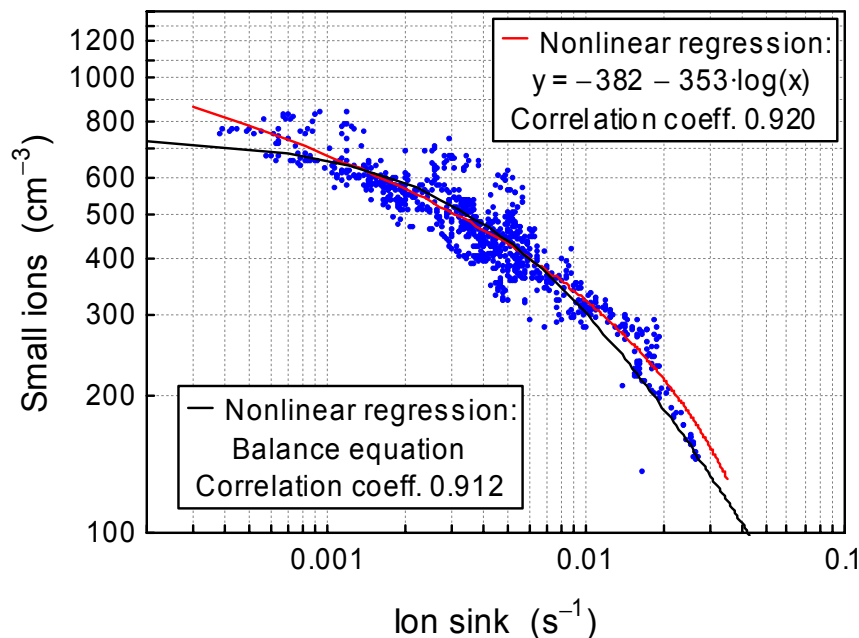
Fig. 4. Scatterplot of the concentration of positive small air ions ( n ) versus ion sink ( S_a ) due to aerosol particles (3–500 nm). Comparison of experimental data and the results derived from the balance equation assuming the ionization rate of 4.8 \text{ ion pairs cm}^{-3} \text{ s}^{-1} , an extra ion loss of 0.0052 \text{ s}^{-1} and the recombination coefficient of 1.5 \times 10^{-6} \text{ cm}^3 \text{ s}^{-1} . Selected data: relative humidity < 95%, wind speed > 1 \text{ m s}^{-1} . 31 March–29 April 1999, Hyttiälä station.
