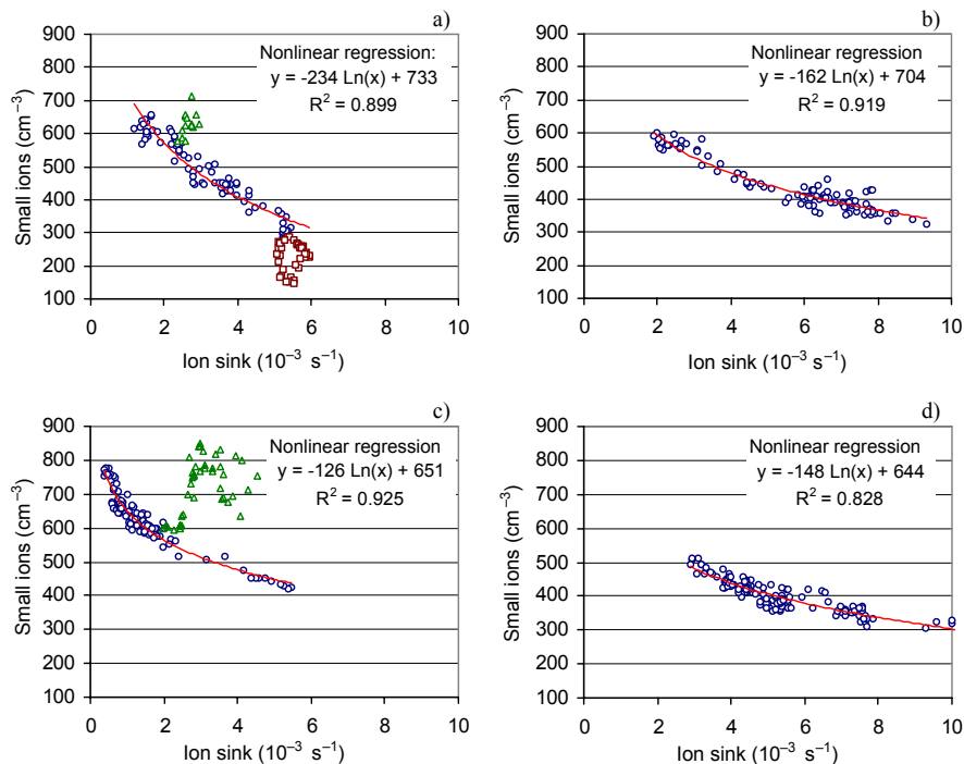
Fig. 9. Scatterplot between the positive small ion concentration and ion sink on 2 April (a), 5 April (b), 10 April (c) and 14 April 1999 (d) at Hyytiälä station. Specific data points: brown squares (□) correspond to the fog event; green triangles (Δ) correspond to the period of weak wind less than 0.2 m s -1 . Specific data points have been excluded from the regression analysis.
