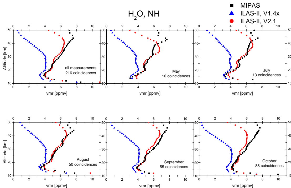
Fig. 1. Comparison of the \text{H}_2\text{O} measurements in the Northern Hemisphere. The mean profiles of the MIPAS-Envisat measurements are shown as black squares, the mean profiles of the ILAS-II V1.4 data as blue triangles and the mean profiles of the ILAS-II V2.1 data as red circles for each month we found coincidences.
