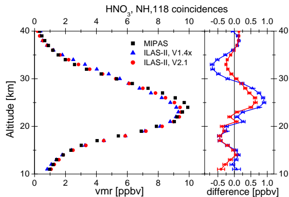
Fig. 10. As in Fig. 2 but for HNO 3 .
