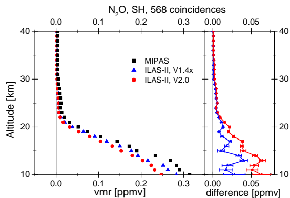
Fig. 16. As in Fig. 14 but for N 2 O.
