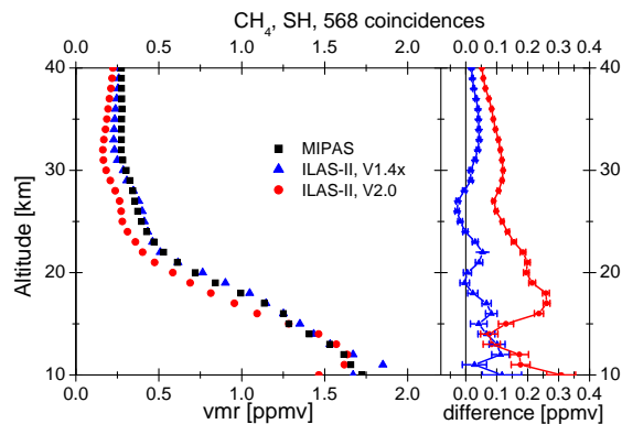
Fig. 18. As in Fig. 14 but for CH 4 .
