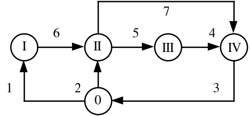
Fig. 1. Nodes and arcs of a graph
