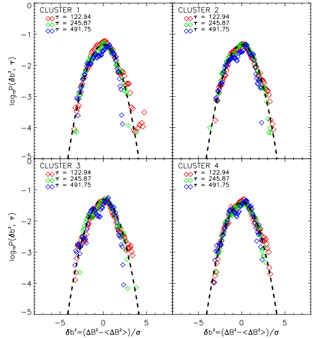
Fig. 5. PDFs of the magnetic energy fluctuations measured by the four Cluster satellites in the cusp at scales larger than \tau_G = 61.47 s; see caption of Fig. 4.
