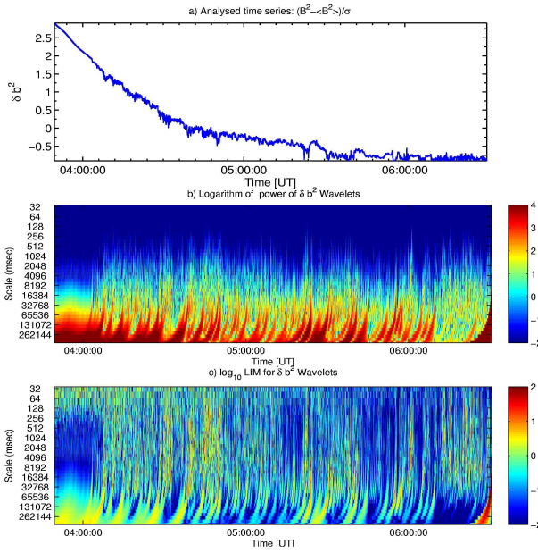
Fig. 8. Haar wavelet analysis of B^2 fluctuations measured by Cluster-1: (a) the analyzed time series; (b) logarithm of the power of \delta b^2 wavelets computed with (4); (c) the local intermittency measure ( LIM ) derived with (5).
