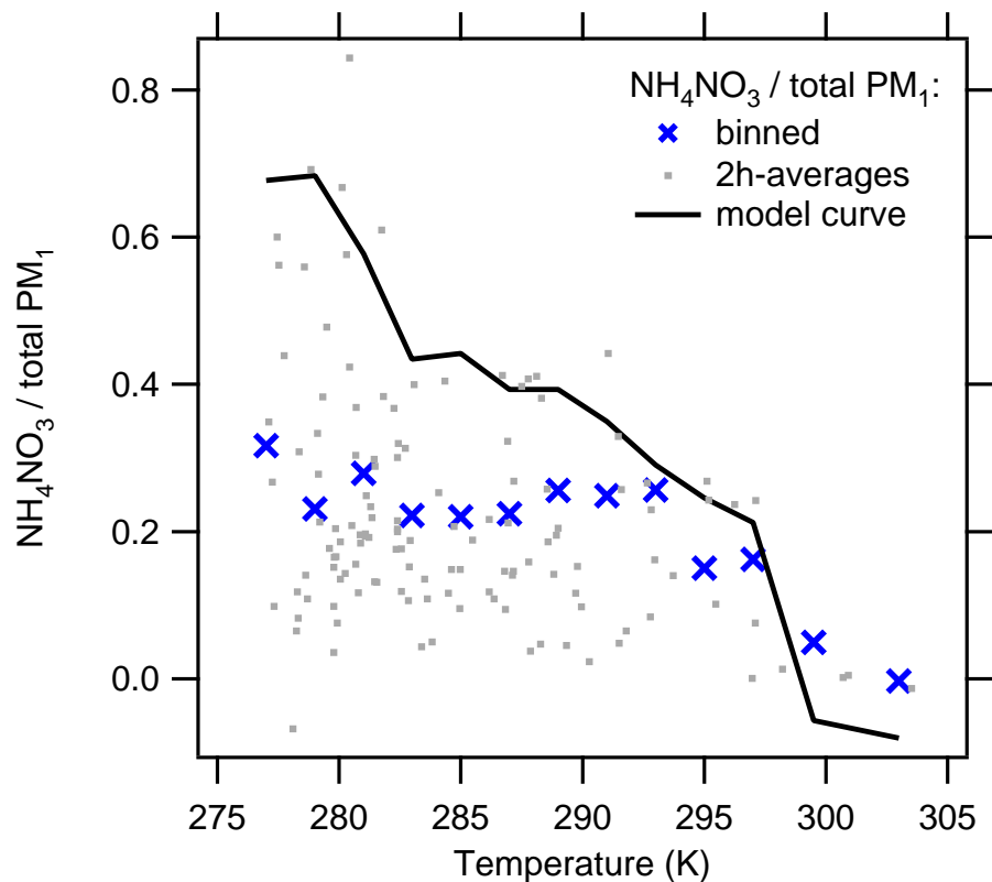
Fig. 5. Measured ratio of NH 4 NO 3 mass concentration to total aerosol mass concentration as a function of temperature, binned into temperature intervals. The dots indicate the two hour averages. The solid represents a model curve with total available nitrate and ammonia as fit parameters (for details see text).
