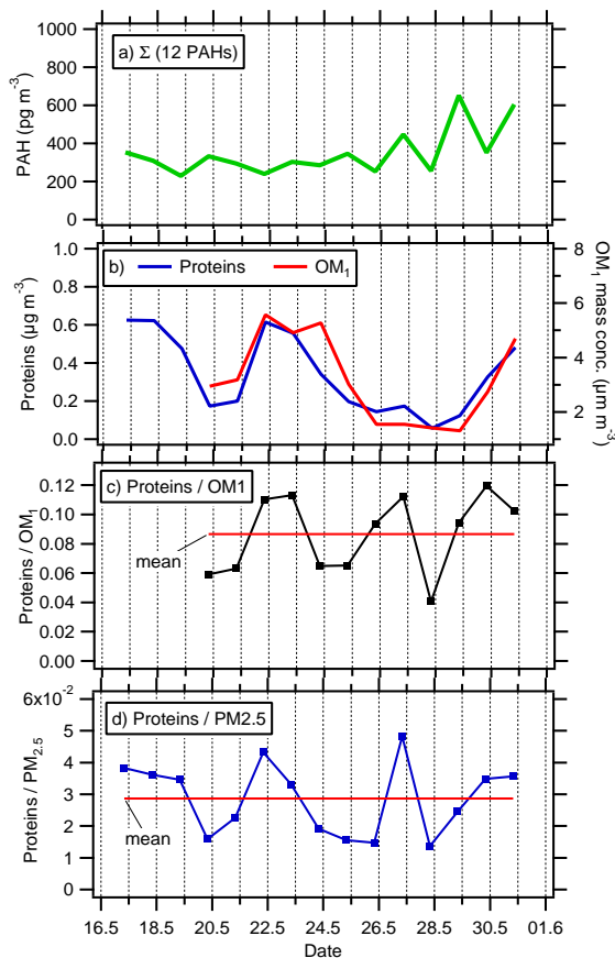
Fig. 9. PAHs und Proteins: (a) Sum of 12 PAHs; (b) Proteins (left scale) along with \text{OM}_1 (right scale); (c) Ratio proteins to \text{OM}_1 (mean: 0.087 \pm 0.027 ); (d) Ratio of proteins to \text{PM}_{2.5} (mean: 0.029 \pm 0.011 ).
