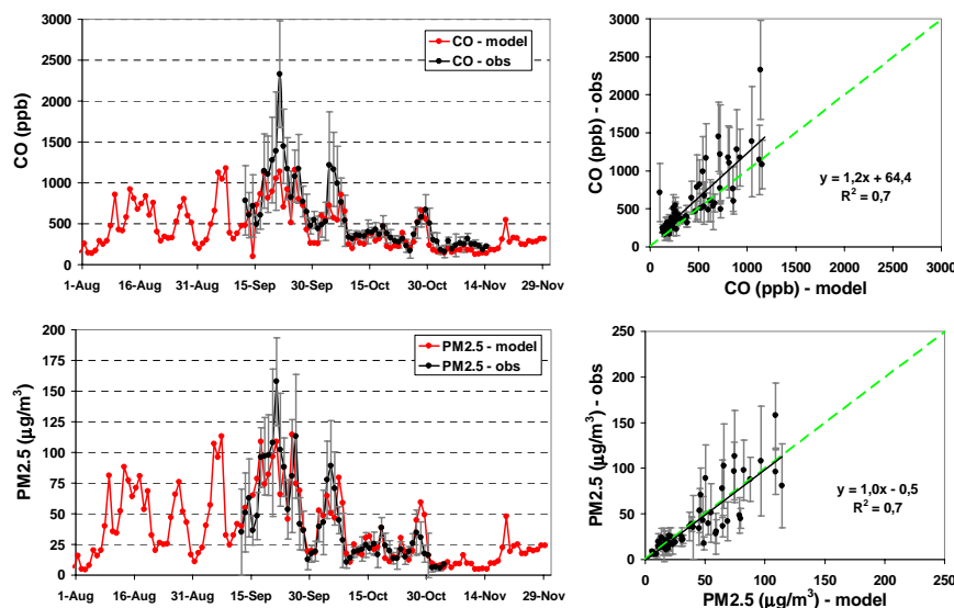
Fig. 13. Time series with comparison between near surface CO (ppb, top) and PM 2.5 (μg m -3 , bottom) observed (black) and model results (red). The measurements were daily averaged and centered at 12:00 Z. The error bars are the standard deviations of the mean values. The model results are presented as instantaneous values at 12:00 UTC.
