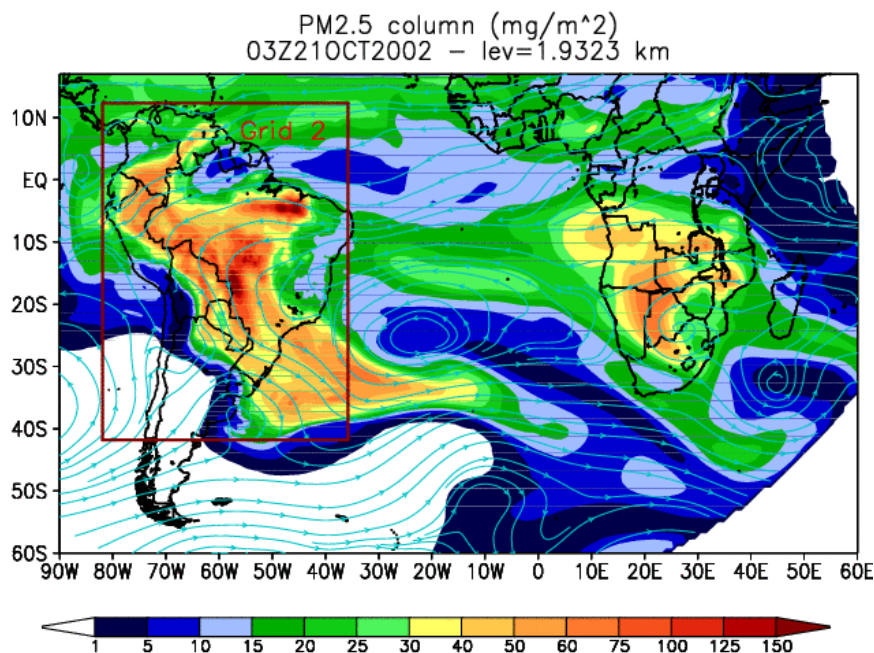
Fig. 3. Particulate material with diameter less than 2.5\mu\text{m} vertically integrated ( \text{mg m}^{-2} ). An example of model results for 03:00 UTC on 21 October 2002 at grids 1 and 2; the red box defines the domain of grid 2 with horizontal resolution of 35 km.
