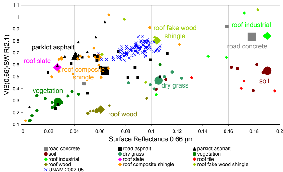
Fig. 3. The ratio between the VIS(0.66 \mu m)/SWIR(2.1 \mu m) is presented as a function of the surface reflectance at 0.66 \mu m , based on the Herald et al. (2003) spectral library. Results from our MODIS analyses are also presented for data analyzed between 2002 and 2005 at 1.5 km resolution over a 10 km box centered on the AERONET site at UNAM in Mexico City.
