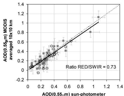
Fig. 5. Aerosol optical depth ( \tau_a ) retrieved from MODIS reflectance data in this study at 1.5\text{ km} \times 1.5\text{ km} resolution and averaged over 10\text{ km} \times 10\text{ km} around the sun-photometer site, compared to \tau_a measured with the sun-photometers averaged over one hour around the satellite overpass time, for \rho_{\text{surf}}(0.66\ \mu\text{m})/\rho_{\text{surf}}(2.1\ \mu\text{m}) values of (a) 0.56 and (b) 0.73. Squares represent data from 2002–2005 from the AERONET at UNAM, and open circles represent data from the sun-photometer network that operated during the MILAGRO Campaign in 2006. The error bars represent their respective standard deviations.
