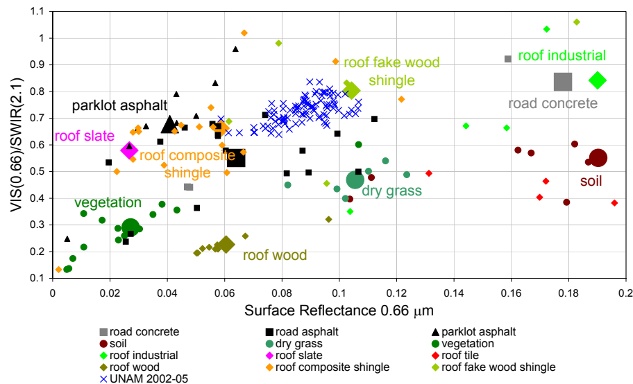
Fig. 3. The ratio between the \text{VIS}(0.66 \mu\text{m})/\text{SWIR}(2.1 \mu\text{m}) is presented as a function of the surface reflectance at 0.66 \mu\text{m} , based on the Herald et al. (2003) spectral library. Results from our MODIS analyses are also presented for data analyzed between 2002 and 2005 at 1.5 km resolution over a 10 km box centered on the AERONET site at UNAM in Mexico City.
