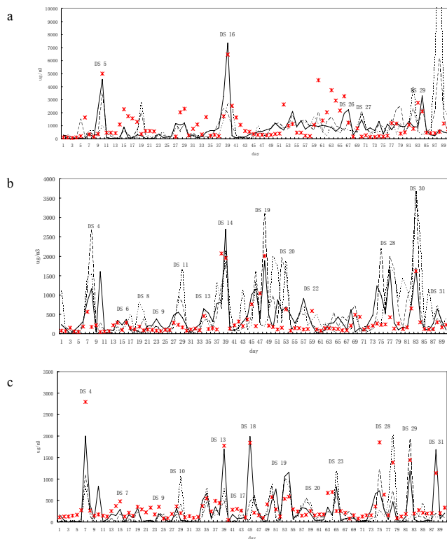
Fig. 6. Comparisons of the surface 24-h mean SDS concentration by 0–24 h (FT1), 24–48 h (FT2) and 48–72 h (FT3) forecasts and the surface PM10 observation for the entire spring from 3 March to 31 May for (a) Tazhong, a station in central part of Taklimakan Deserts in Xinjiang province in China, (b) for Ejilaqi, a station in the north of Badain Juran deserts, (c) for Zhurihe, a station in the west of Onqin Daga sandy areas, (d) for Beijing, a station away from SDS source area, and (e) for Dalian, a station away from SDS source areas and in the west coast of the Bohai sea, respectively. DS xx, such as DS 4, means dust event number defined in Table 1.
