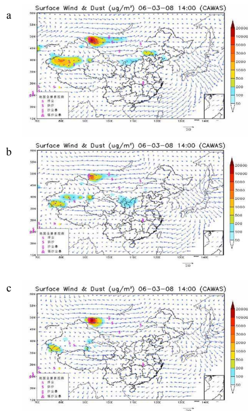
Fig. 1. Surface snap SDS concentrations and wind field at 14 h on 8 March at forecast length of (a) 54, (b) 30 and (c) 6 h from the initial forecast time of 8 h on 6, 7 and 8 March, respectively (Beijing standard time used). The scattered pink signals S, $, § and & represent observation records of suspended dust, blowing dust, SDS and severe SDS respectively from weather stations at the same time with the concentration plot.
