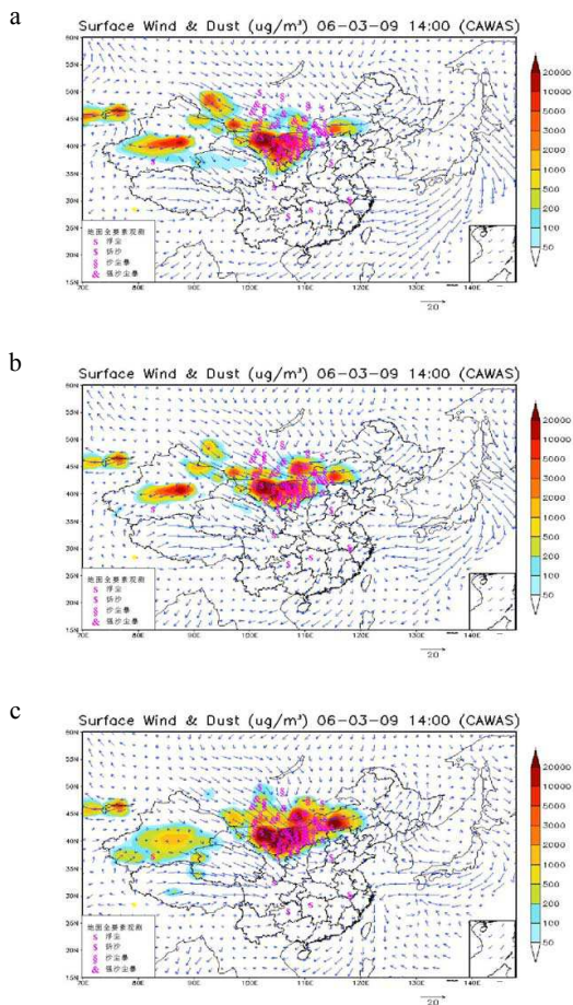
Fig. 2. Surface snap SDS concentrations and wind field at 14 h on 9 March at a forecast length of (a) 54, (b) 30 and (c) 6 h from the initial forecast time of 8 h on 6, 7 and 8 March, respectively (Beijing standard time used).
