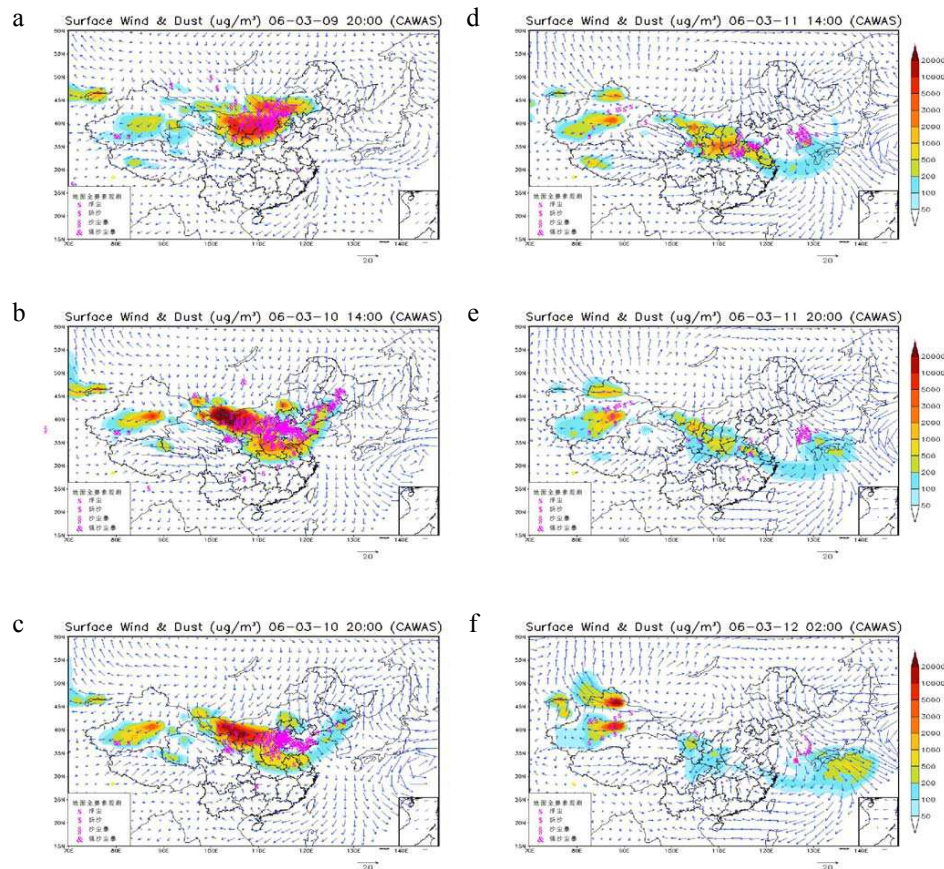
Fig. 4. Surface snap SDS concentrations and wind field at (a) 20 h on 9 March, (b) 14 hr on March 10, (c) 20 h on 10 March, (d) 14 h on 11 March, (e) 20 h on 11 March, and (f) 2 h on 12 March (local time used) from the initial forecast time of 8 h on 9 March (Beijing standard time used).
