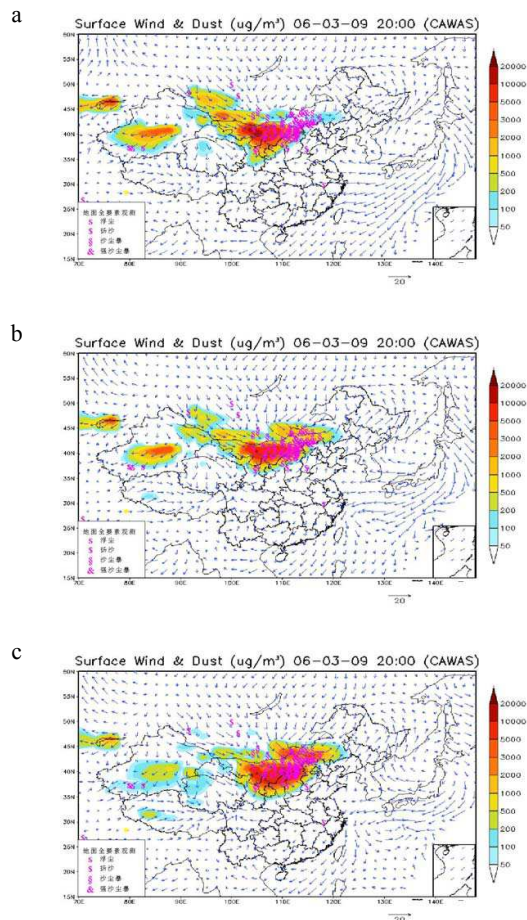
Fig. 3. Surface snap SDS concentrations and wind field at 20 h on 9 March at a forecast length of (a) 60 (b) 36 and (c) 12 h from the initial forecast time of 8 h on 7, 8 and 9 March, respectively (Beijing standard time used used).
