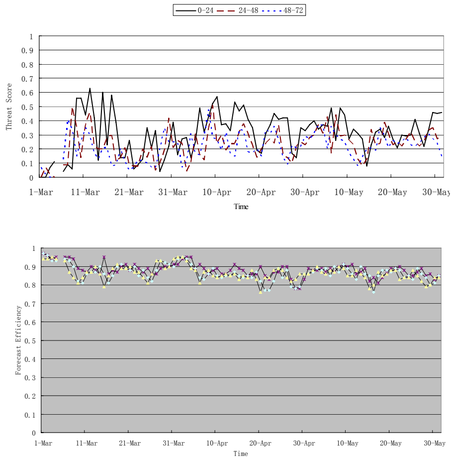
Fig. 7. Threat Scores (upper) and accuracy (lower) of 0–24 h, 24–48 h and 48–72 h forecasts for CUACE/Dust in 2006 spring.
