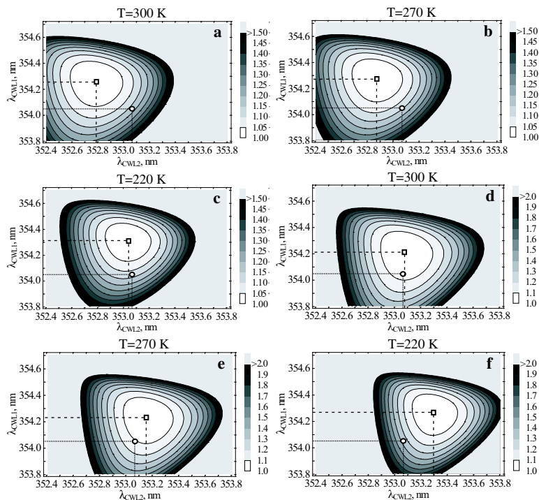
Fig. 3. Results of the optimization calculations for the parameters of the rotational Raman channel filters: Calculated statistical temperature uncertainty \Delta T versus filter CWLs \lambda_{\text{CWL1}} and \lambda_{\text{CWL2}} for the filters shown in Fig. 2. Left: (a) (T_1, T_2) = (300 \text{ K}, 305 \text{ K}) , (b) (T_1, T_2) = (270 \text{ K}, 275 \text{ K}) and (c) (T_1, T_2) = (220 \text{ K}, 225 \text{ K}) . Right: same as (a–c) but with a background signal of the same intensity as the strongest rotational Raman line in the anti-Stokes branch added to the signals. Calculation step width was 0.01 nm. Values for \Delta T are scaled relatively to the minimum ( \square ) of each plot. The circle marks our setup. The gray scale of \Delta T is plotted on the right.
