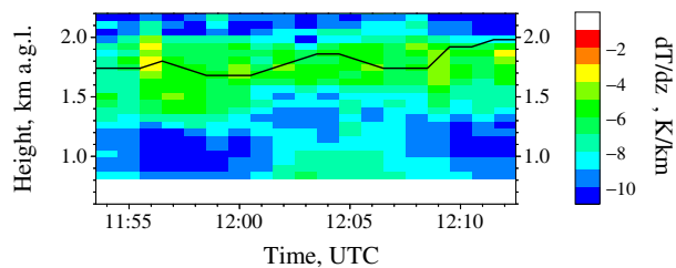
Fig. 8. Time-height cross section of the temperature gradient on 23 March 2006 at University of Hohenheim (Stuttgart, Germany). The black line is marking the boundary layer top derived by Fig. 7.
