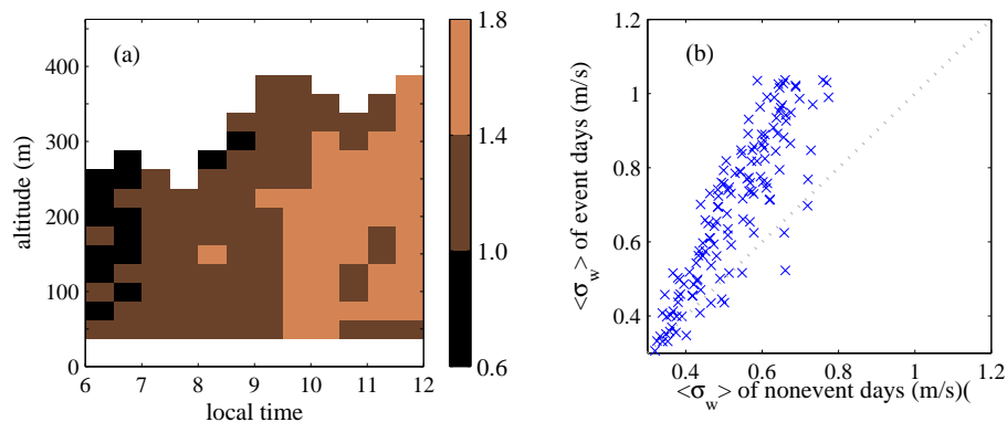
Fig. 4. (a) The ratio of event day values and nonevent day values of \langle \overline{\sigma_w} \rangle(t, z) and (b) the event day values (Fig. 3b) vs. the nonevent day values (Fig. 3a). The dotted line is 1:1-relationship.
