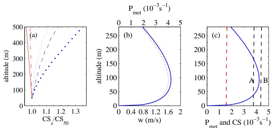
Fig. 5. (a) The influence of increase of RH (dashed curve), decrease of T (dash-dotted curve) and decrease of dN_z/d \log D_p (solid curve) on CS in an ascending air parcel. The total effect is represented by a dotted curve and the profiles are based on surface measurements on 29 March 2003. The dots are mean values for all the studied data and all the values have been scaled by CS_{50\text{m}} . (b) The theoretical P_{\text{met}} profile (solid curve) based on a parametrized vertical velocity profile (dotted curve) and surface measurements on 29 March 2003 ( \theta=276\text{ K} , z_i=327\text{ m} , \overline{w'\theta'_s}=0.04\text{ m s}^{-1}\text{ K} ). (c) P_{\text{met}} (blue solid curve) and CS (red dashed curve), which is based on measurements and two theoretical profiles of CS (dashed curves A and B).
