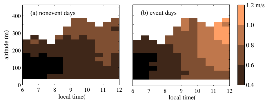
Fig. 3. The average standard deviation of vertical velocity \langle \overline{\sigma_w} \rangle(t, z) on (a) the nonevent days and (b) event days observed by the sodar in Hyytiälä.
