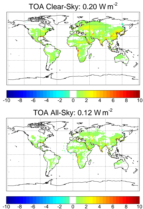
Fig. 9. Annual-mean difference of clear-sky and all-sky anthropogenic direct aerosol radiative forcings between simulations applying the upper (ALB-H) and lower (ALB-L) bound of the AeroCom land surface albedos given in Fig. 8.
