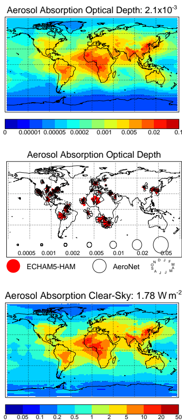
Fig. 3. ECHAM5-HAM simulated BASE year 2000 mean clear-sky aerosol absorption optical depth [1] at wavelength \lambda = 550 \text{ nm} , comparison of simulated (red) and AERONET sun-photometer retrieved (black) clear-sky aerosol absorption optical depth [1] as seasonal distribution (clockwise, starting at 12 o'clock) at respective AERONET locations, simulated clear-sky short-wave aerosol absorption [ \text{W m}^{-2} ]. Global annual-mean values are given in the titles.
