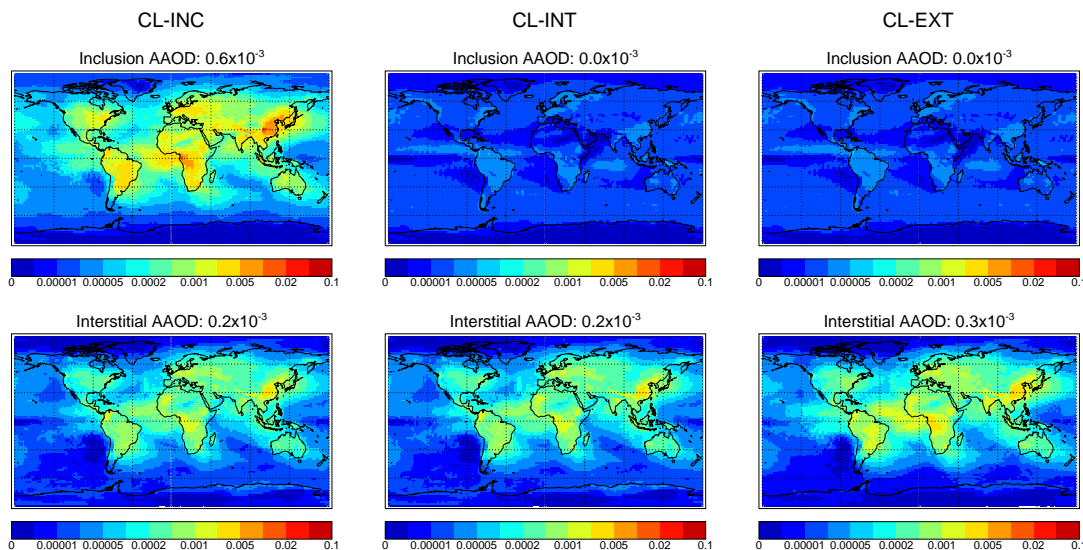
Fig. 12. Annual-mean in-cloud broad-band visible (0.25–0.69 μm) aerosol absorption optical depths from the CL-INC, CL-INT, and CL-EXT simulations, integrated over the cloudy layers of the atmospheric column. Inclusion AAOD: inclusion aerosol AAOD, i.e. cloud absorption optical depth with consideration of black carbon inclusions; Interstitial: interstitial AAOD.
