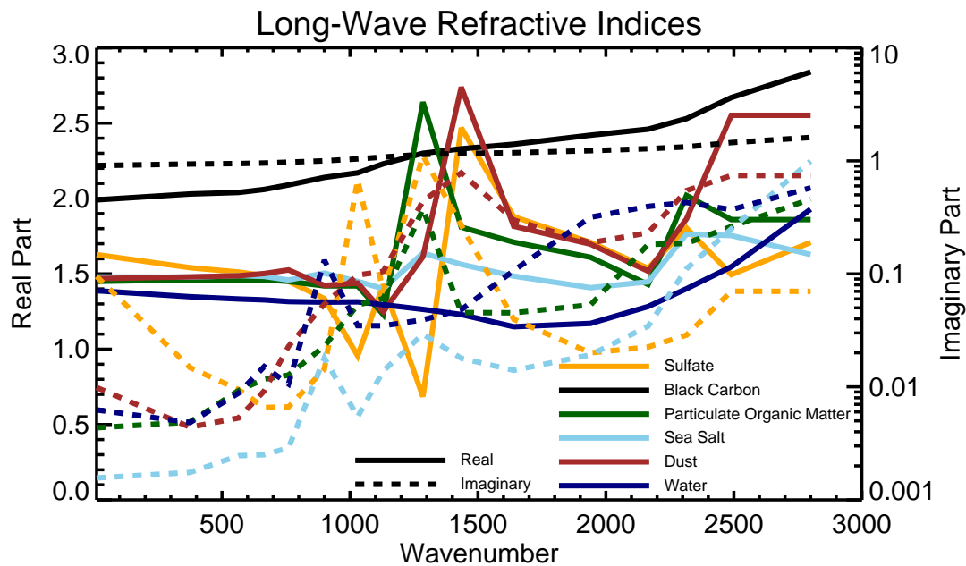
Fig. 1. Long-wave component refractive indices as given in Table 4.
