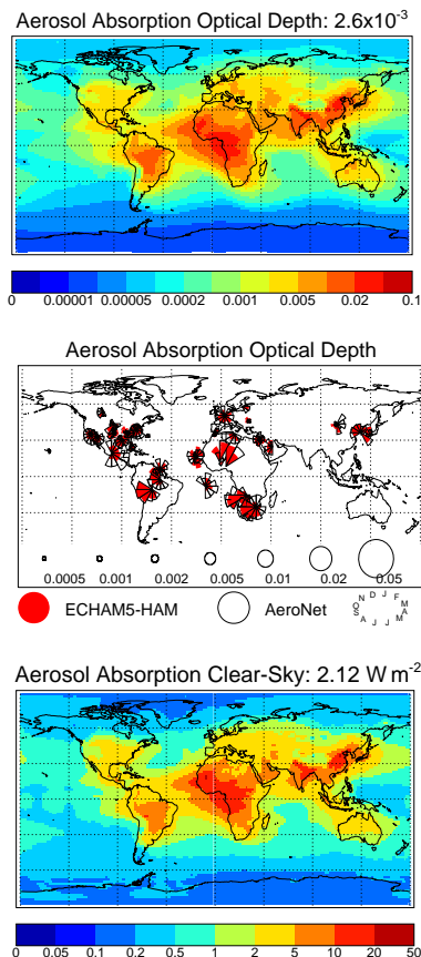
Fig. 6. ECHAM5-HAM simulated BRUG year 2000 mean clear-sky aerosol absorption optical depth [1] at wavelength \lambda = 550 \text{ nm} , comparison of simulated (red) and AERONET sun-photometer retrieved (black) clear-sky aerosol absorption optical depth [1] as seasonal distribution (clockwise, starting at 12 o'clock) at respective AERONET locations, simulated clear-sky short-wave aerosol absorption [ \text{W m}^{-2} ]. Global annual-mean values are given in the titles.
