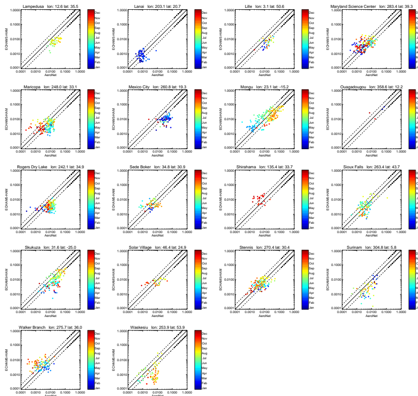
Fig. A1. Continued. Scatterplots of year 2000 daily-mean ECHAM5-HAM simulated and AERONET retrieved absorption optical depth at wavelength \lambda = 550 nm for the BB-M simulation as used in Fig. 4b). The ECHAM5-HAM output is sampled for each measurement date at the model grid box containing the measurement station. The seasonality is colour coded.
