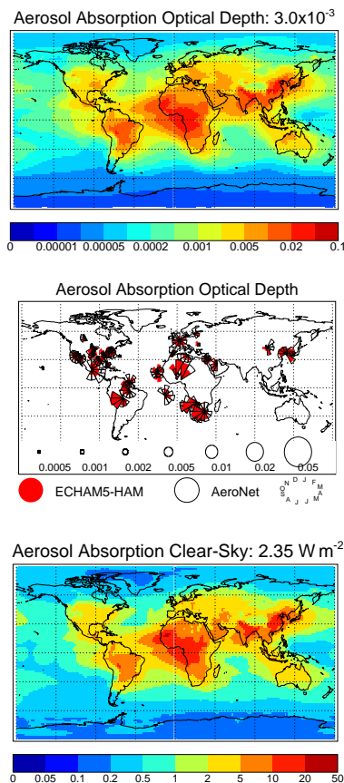
Fig. 4. ECHAM5-HAM simulated BB-M year 2000 mean clear-sky aerosol absorption optical depth [1] at wavelength \lambda = 550 \text{ nm} , comparison of simulated (red) and AERONET sun-photometer retrieved (black) clear-sky aerosol absorption optical depth [1] as seasonal distribution (clockwise, starting at 12 o'clock) at respective AERONET locations, simulated clear-sky short-wave aerosol absorption [ \text{W m}^{-2} ]. Global annual-mean values are given in the titles.
