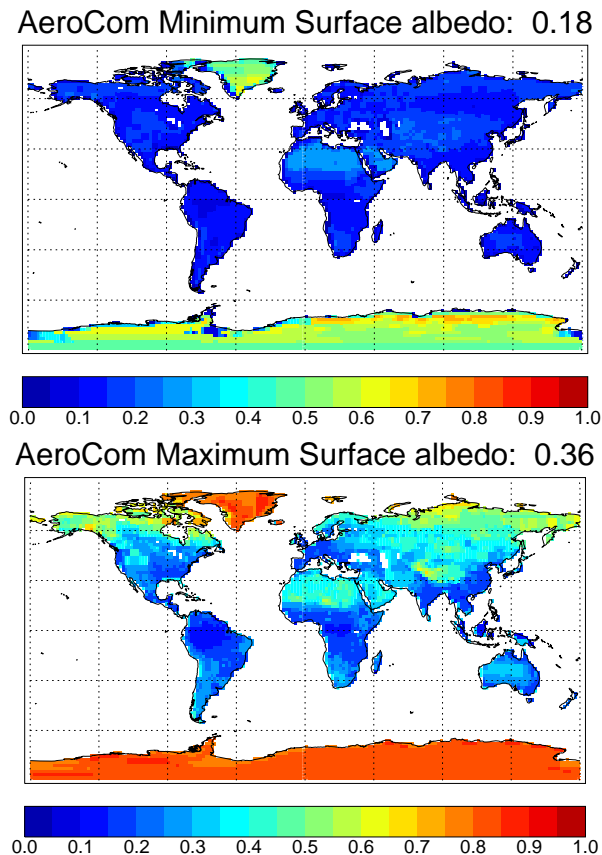
Fig. 2. Global distribution and mean of the upper and lower bound of broadband short-wave ( 0.2\text{--}4.0\ \mu\text{m} ) land surface albedo fields sampled from submissions the AeroCom forcing experiment.
