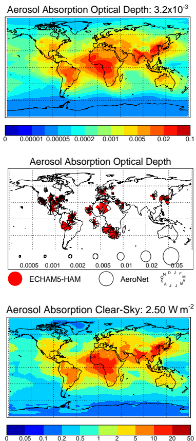
Fig. 5. ECHAM5-HAM simulated BB-H year 2000 mean clear-sky aerosol absorption optical depth [1] at wavelength \lambda = 550 \text{ nm} , comparison of simulated (red) and AERONET sun-photometer retrieved (black) clear-sky aerosol absorption optical depth [1] as seasonal distribution (clockwise, starting at 12 o'clock) at respective AERONET locations, simulated clear-sky short-wave aerosol absorption [ \text{W m}^{-2} ]. Global annual-mean values are given in the titles.
