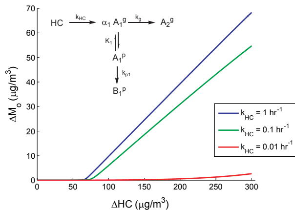
Fig. 8. Effect of HC oxidation rate ( k_{\text{HC}} ) on SOA growth in case (b) with fast (blue), medium (green) and slow (red) hydrocarbon oxidation. k_{\text{g}}=k_{\text{p}1}=1 \text{ h}^{-1} , \alpha_1=0.3 , K_1=0.05 \text{ m}^3/\mu\text{g} , M_o(0)=0.01 \mu\text{g}/\text{m}^3 .
