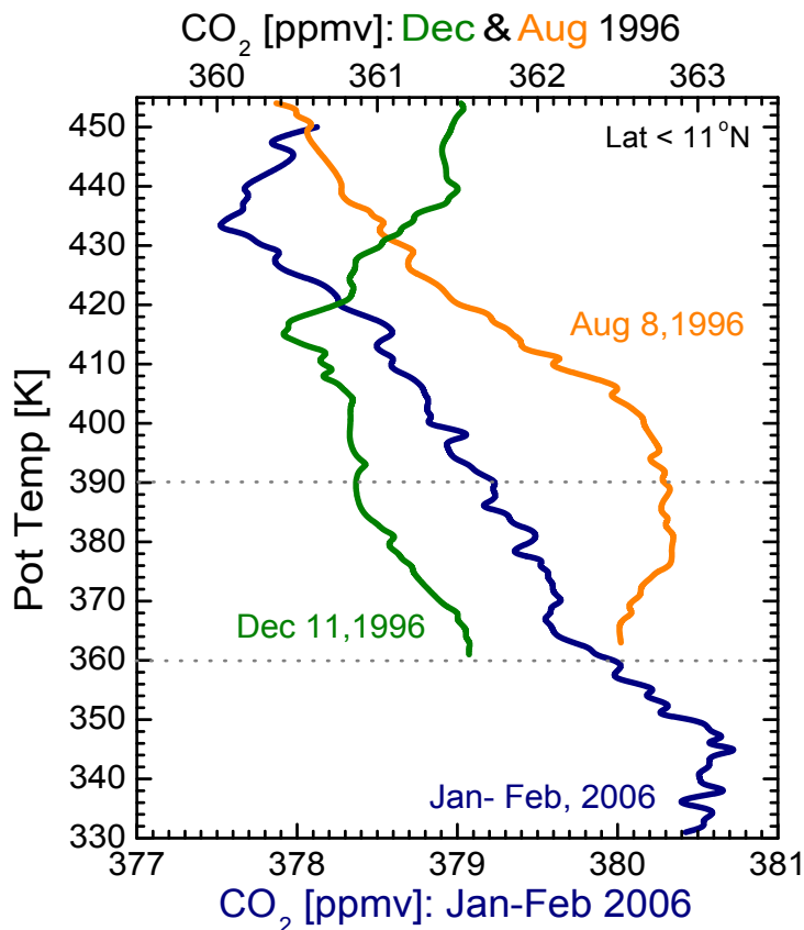
Fig. 10. Two profiles of CO 2 in the TTL from the central Pacific obtained during STRAT are shown along with CR-AVE CO 2 . Data from winter (December) are remarkably consistent with data from CR-AVE. Note the reversed CO 2 gradient in August and thus operation of the CO 2 clock.
