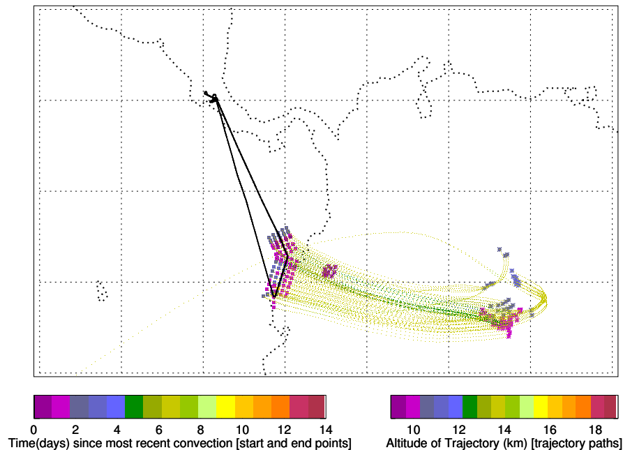
Fig. 7. Back trajectories that trace the low-CO 2 air masses at ~350 K of the flight on 9 February 2006 to Amazon basin.
