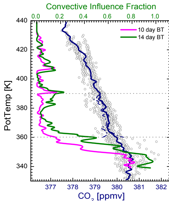
Fig. 9. Vertical profiles of CR-AVE CO 2 and fraction of air cluster points with non-zero convective influence, which was calculated by back trajectory analyses to convective systems, based on the method of Pfister et al. (2001). The pink and green lines show the 1-K averaged fraction of air clusters influenced by convection for 10 day and 14 day trajectories, respectively. To test the degree of convective influence on CO 2 distribution, CR-AVE CO 2 profile between 360 and 390 K is corrected for convective influence fraction of 10 day back trajectory. Convective air flux is assumed of two versions of CO 2 mixing ratios: 378.5 and 383 ppmv that are lower and upper limits. The corrected profiles are represented by dotted line (see text in Sect. 3.3.2). Symbols for CO 2 are same as in Fig. 8.
