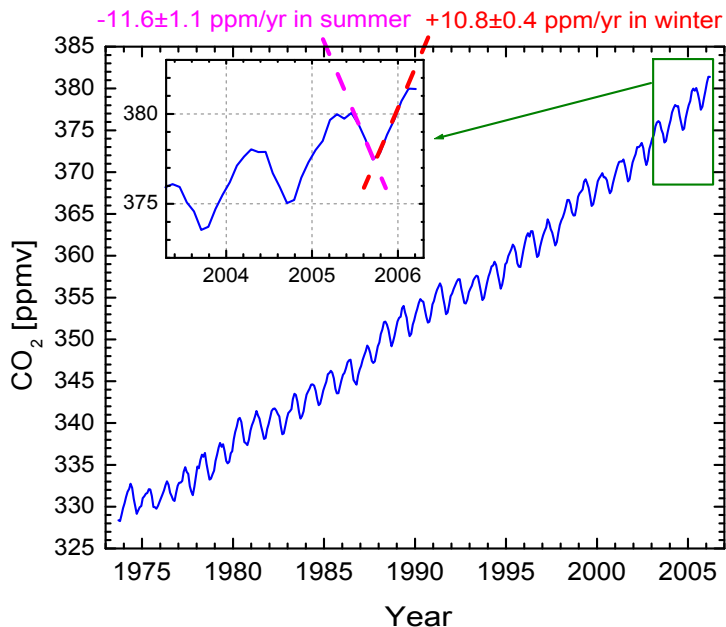
Fig. 1. The global CO 2 seasonal cycle from (\text{CO}_2\text{-MLO} + \text{CO}_2\text{-SMO})/2 (Boering et al., 1996) using ESRL data (Conway et al., 1994, updated by T. Conway). The inset shows an expanded time axis with the CR-AVE time period.
