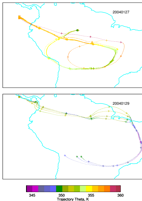
Fig. 6. Back trajectories that trace (a) the low-CO 2 air masses at \sim 360 K of the flight on 27 January and (b) the air mass at \sim 350 K of the flight on 29 January to Amazônia.
