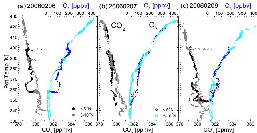
Fig. 3. Vertical profiles of CO 2 (denoted by solid dots) and O 3 (by blue diamonds) on 6(a), 7(b), and 9(c) February. Low CO 2 bulges from <math>< 5^{\circ}\text{N}</math> are responding to high ozone signals, suggesting stratospheric air input. Note dotted circle on 9 February marks the air mass influenced from deep convection over Amazon basin, discussed in Sect. 3.2.2.
