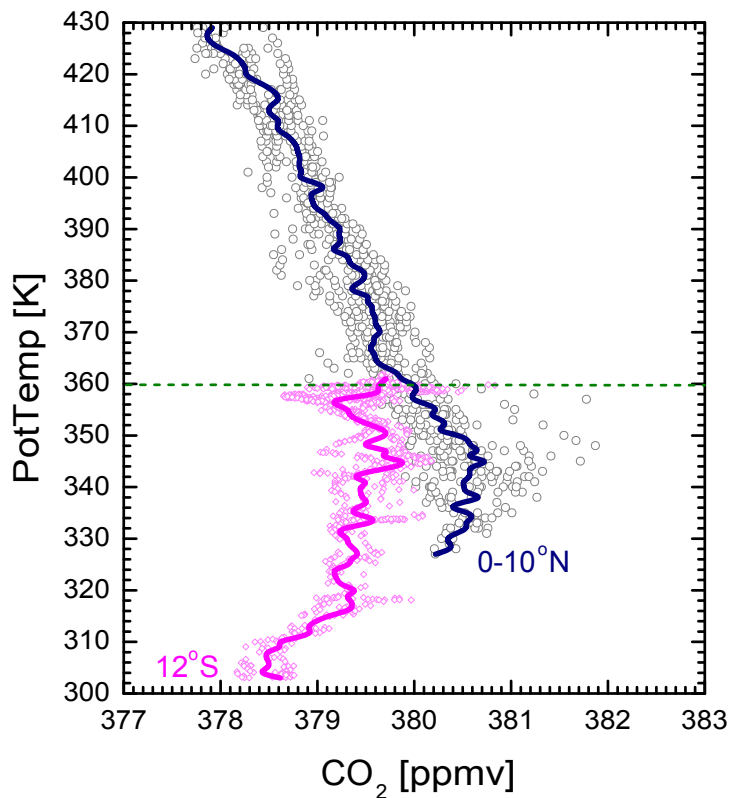
Fig. 8. Vertical profiles of \text{CO}_2 obtained during CR-AVE and TWP-ICE. TWP-ICE observations were plotted from \sim 1 -km to 15-km altitude on 25, 27, and 29 January 2006. The measurements were performed over the Western Pacific ocean ( 12^\circ \text{S} , 130^\circ \text{E} ). All the data were averaged into 1-K intervals for each flight. Empty cycle denotes CR-AVE \text{CO}_2 and empty diamonds for TWP-ICE \text{CO}_2 . The overall 1-K averages for each mission are also shown in solid lines.
