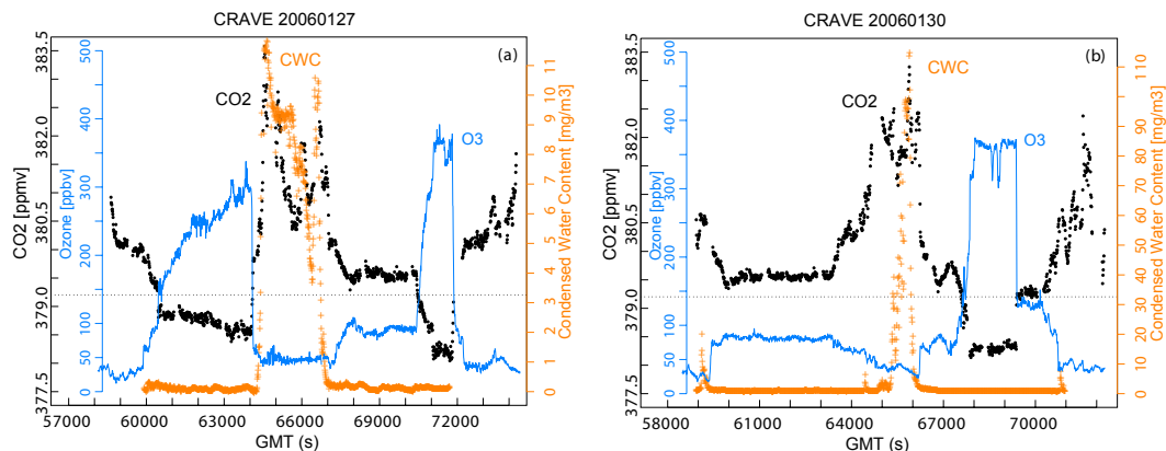
Fig. 4. Flight segments for CO 2 , O 3 and condensed water content (CWC) (a) on 27 January and (b) on the 30th. The CO 2 peaks that correspond to CO 2 spikes in the vertical profiles (Figs. 2e and 2f), are clearly responding to enhanced condensed water content in the outflow of convective clouds. Note high O 3 and low CO 2 mixing ratios on the stratospheric side. Horizontal dotted line represents a CO 2 level at the tropopause. Black, solid dots give CO 2 , blue lines for O 3 , and orange, cross symbols for CWC.
