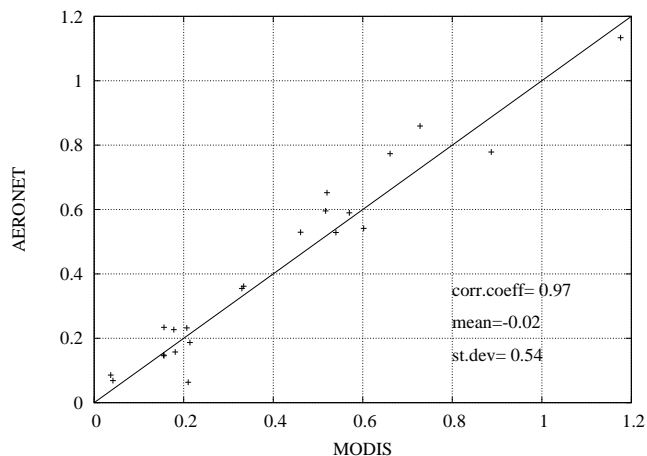
Fig. 2. Scatter plot of MODIS and AERONET AOD at 0.55 \mu\text{m} for Tõravere. The mean and standard deviation are calculated from the difference of MODIS and AERONET AOD, divided by AERONET AOD [i.e. (\text{MODIS}-\text{AERONET})/\text{AERONET} ].
