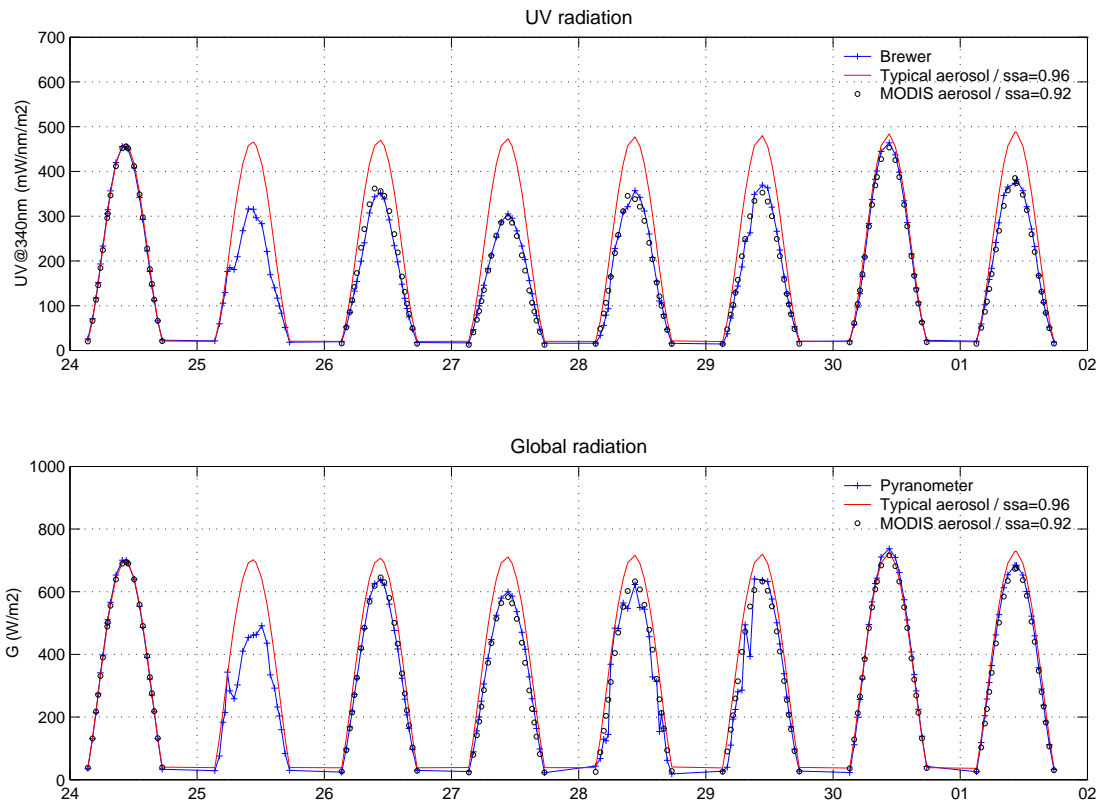
Fig. 8. Measured irradiances together with irradiances simulated using different aerosol settings: (upper panel) UV irradiances at 340 nm, (lower panel) global irradiances. MODIS data for 25 April were not available.
