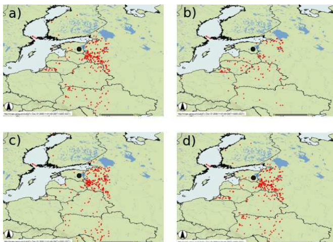
Fig. 4. MODIS Firemapper detection for the following days (a) 28 April, (b) 29 April, (c) 30 April, (d) 1 May. Tõravere is indicated by a black dot.
