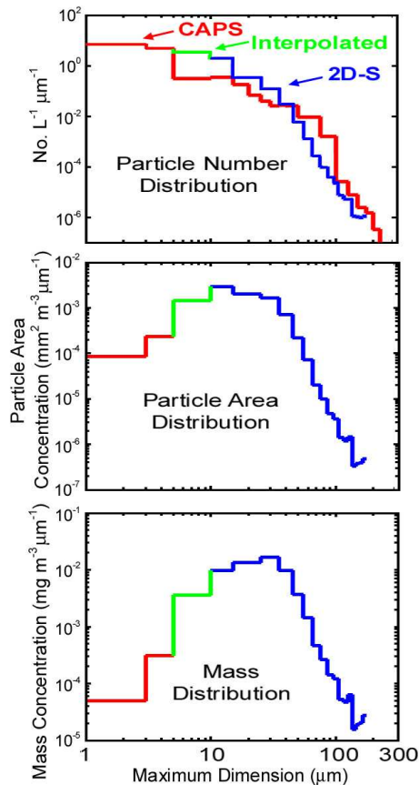
Fig. 9. PSD's of (top) number concentration, (middle) area and (bottom) mass based on \sim 1800 km of WB-57F 2D-S and CAPS measurements collected in SVC. Green trace is interpolated between 5 \mu\text{m} CAS and 10 \mu\text{m} 2D-S size bins.
