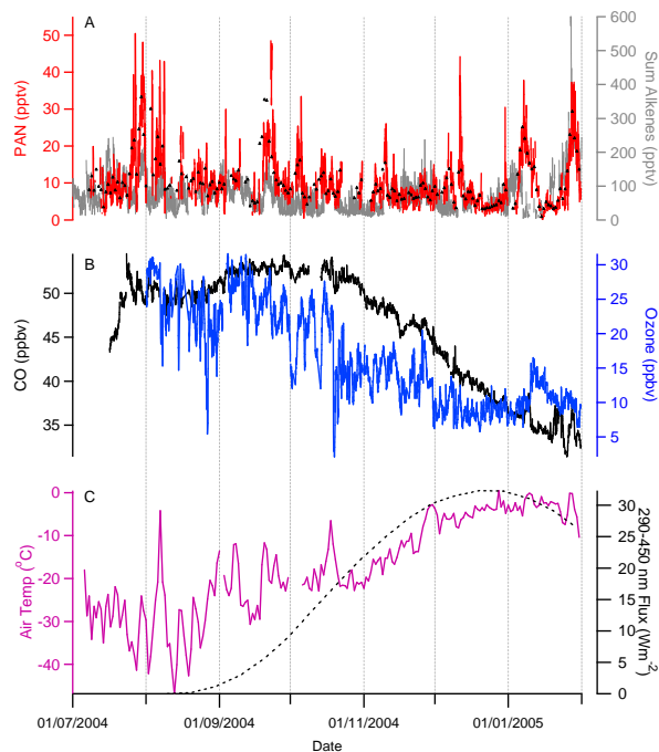
Fig. 3. Timeseries of data from Halley from July 2004 to Feb 2005 showing (A) hourly PAN measurements (red line) , daily mean PAN mixing ratios (black triangles) and the \Sigma_{C_2-C_5} alkenes. (B) ozone (blue) and CO (black) hourly measurements (C) hourly air temperature (red) and TUV calculated irradiation (290–450 nm) as a guide to photochemically active radiation.
