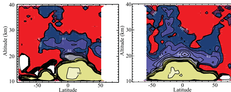
Fig. 3. CALIPSO stratospheric 532-nm aerosol backscatter profiles for (a) 2 July 2006 and (b) 7 January 2007. Red regions have aerosol backscatter less than zero, while white areas showing missing values. The contour values are 0, 0.001, 0.01, 0.1, 0.2, 0.4, 0.6, 0.8, 1, 2, 4, 6, 8, 10, and 100 for aerosol backscatter coefficient in \text{km}^{-1} \text{str}^{-1} times 10^5 . Areas in the troposphere with extinction coefficient values greater than 10^{-4} \text{km}^{-1} \text{str}^{-1} are strongly influenced by the presence of cloud.
