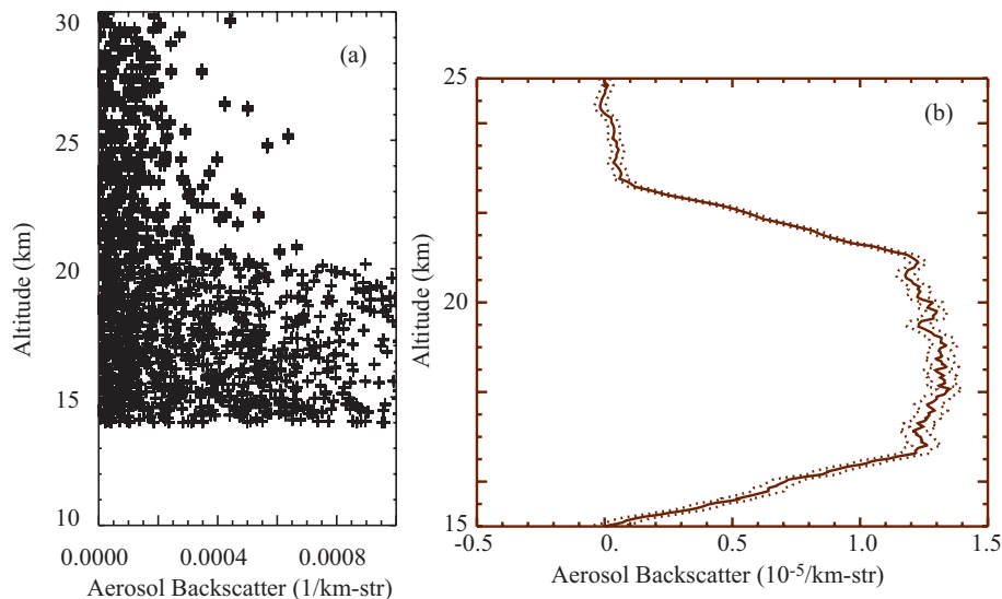
Fig. 2. (a) A depiction of 100 individual simulated CALIPSO 532-nm backscatter profiles for a “top hat” stratospheric layer between 16 and 22 km. The abrupt change in noise at 20 km is due to a change in on-board smoothing and not due to any atmospheric signal. (b) Simulated retrieval of a stratospheric aerosol layer using CALIPSO backscatter data. This profile is a 1-day, 5-deg latitudinal average for background conditions.
