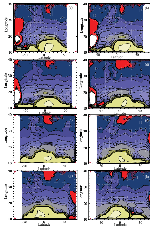
Fig. 6. Cross sections of CALIOP aerosol attenuated backscatter at 532 nm where the total backscatter has been adjusted by +5% for (a) 2 July 2006, (b) 6 August 2006, (c) 3 September 2006, (d) 1 October 2006, (e) 5 November 2006, (f) 3 December 2006, (g) 7 January 2007, and (h) 4 February 2007. Red regions have aerosol backscatter less than zero, while white areas showing missing values. The contour values are 0, 0.001, 0.01, 0.1, 0.2, 0.4, 0.6, 0.8, 1, 2, 4, 6, 8, 10, and 100 for aerosol backscatter coefficient in \text{km}^{-1} \text{str}^{-1} times 10^5 . Areas in the troposphere with extinction coefficient values greater than 10^{-4} \text{km}^{-1} \text{str}^{-1} are strongly influenced by the presence of cloud. Areas within either winter time polar vortex, known to have very low aerosol content, are found to have backscatter coefficient values less than 0.
