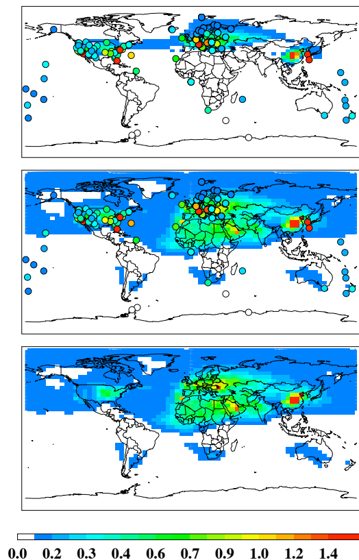
Fig. 2. Annual mean surface concentrations of ammonium-nitrate. The filled circles show measurements as observed by the EMEP, IMPROVE and the Prospero network. The upper panel shows fine mode nitrate aerosol, the middle panel fine and coarse mode nitrate, and the lower panel shows fine and coarse mode nitrate, but excluding the observations. Units are in [\mu\text{g m}^{-3}] .
