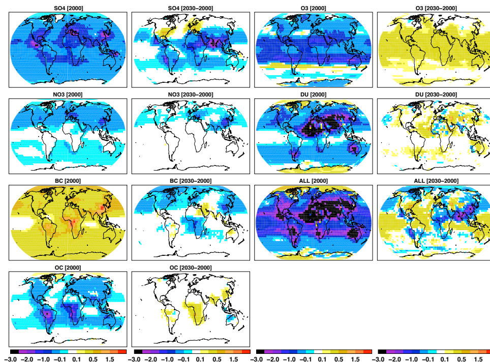
Fig. 10. Top of the atmosphere radiative forcings [W/m 2 ] of each individual aerosol species (fine mode sulphate (SO 4 ) and nitrate (NO 3 ), black (BC) and organic (OC) carbon, mineral dust (DU) and ozone (O 3 ). The maps entitled “ALL” shows the sum of all aerosols and gases, the net forcing. The forcings are shown for the year 2000 and the differences between 2030 and 2000.
