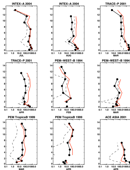
Fig. 5. Vertical profiles of ammonium-nitrate concentrations in [ppt_v] as observed during various field campaigns by the DC8 air plane (black line), compared to the models total (fine and coarse mode) ammonium-nitrate (red line) and its fine mode fraction (black dotted line) only. The title shows the name and the year or the campaign, and the subtitle the month. INTEX-A covers Eastern U.S. (Singh et al., 2006), TRACE-P the North Hemispheric Western Pacific (Jacob et al., 2003), PEM-WEST-B the Western Pacific (Hoell et al., 1997), PEM-Tropics the Southern Pacific (Raper et al., 2001) and ACE-ASIA East Asia and the Northern Pacific (Huebert et al., 2003). The model date are interpolated to the flight tracks and then the monthly mean vertical profiles are calculated.
