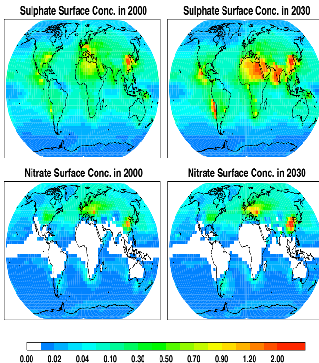
Fig. 7. Annual mean near surface concentrations of fine mode sulphate (upper panel) aerosols and nitrate (lower panel) for the year 2000, and 2030. Units are in [\mu\text{g}/\text{m}^3] .
