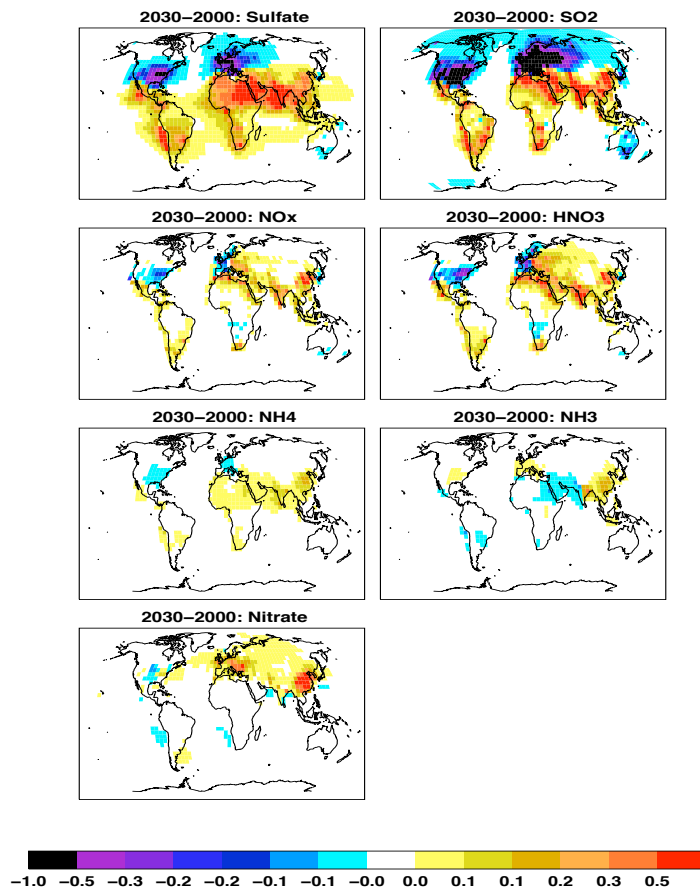
Fig. 6. Difference between the years 2030 and 2000 in near surface concentrations, in [\mu\text{g}/\text{m}^3] , of SO 2 , NO x , HNO 3 , NH 4 , NH 3 and fine mode nitrate.
