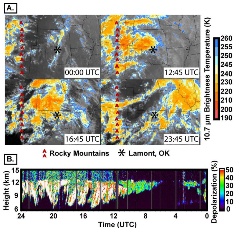
Fig. 1. Infrared satellite and lidar depolarization observations on 19 April 2001: (A) GOES infrared satellite image time series. Low brightness temperatures indicate high cloud tops. (B) Vertically pointing lidar depolarization ratio observations from Lamont. High depolarization ratios (>10%) indicate ice.
