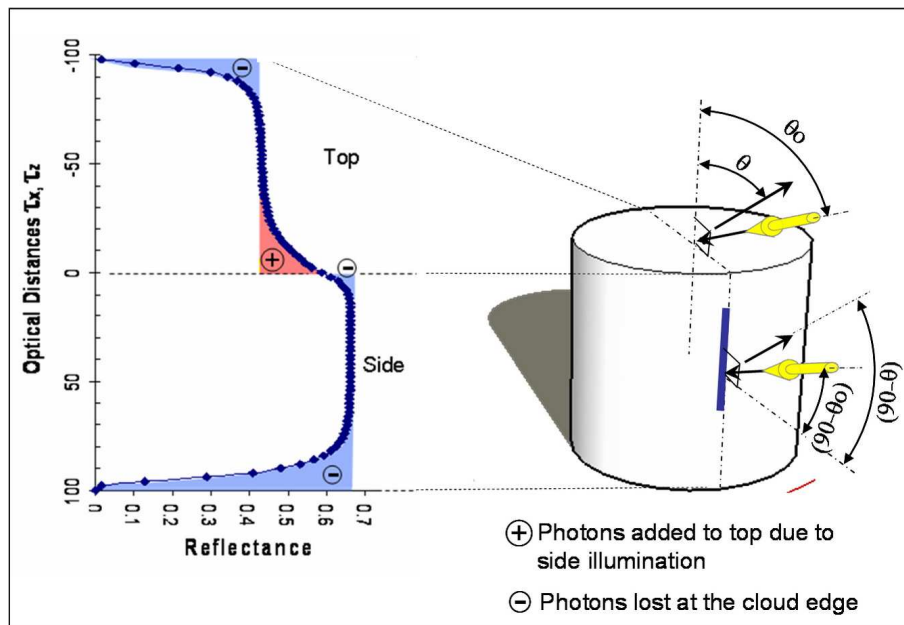
Fig. 4. Cloud side and top radiances at 2.1\ \mu\text{m} calculated with the 3-D radiative transfer code SHDOM for a simplified cylindrical cloud with homogeneous r_{\text{eff}}=10\ \mu\text{m} water droplets, solar zenith angle \theta_0=60^\circ , and view zenith angle \theta=45^\circ . The colored (blue and red) areas around the plot represent photons been added or lost near the cloud edges. In this particular case the top reflectance is lower than the side reflectance due to the relative angle between the solar illumination and a vector normal to the side or the top surfaces. The relative angle with the top surface vector is 60^\circ whereas the angle with the side vector is 30^\circ . The blue line along the surface of the cylinder represents the region where there is saturation and the 2.1\ \mu\text{m} reflectance from the cylinder equals a plane parallel result with the proper geometry. A point half way along the blue line represents the general place that was selected to construct our 3-D look-up-table from retrievals away from the cloud edges. Other regions of the cylinder could be used for retrievals closer to cloud base or top.
