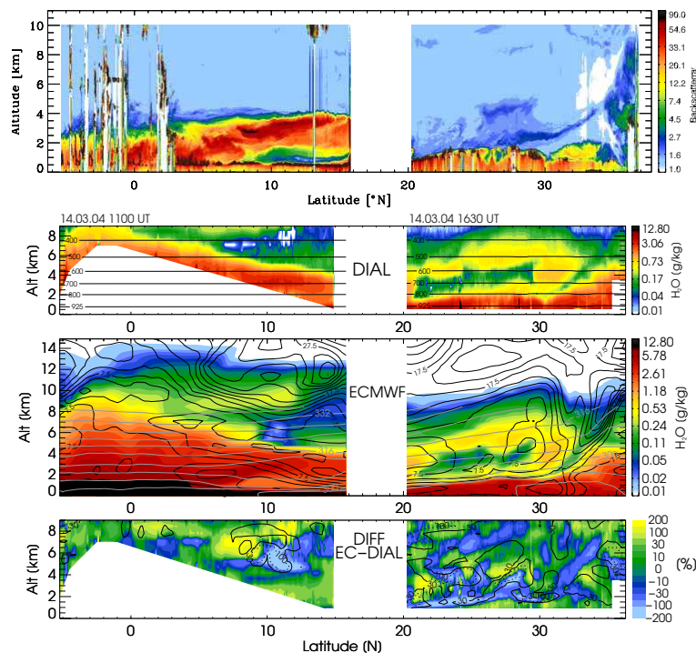
Fig. 3. Backscatter ratio R (a) and water vapour mixing ratio q in g/kg (b) along DIAL flights on 14 March 2004, 11:00–14:00 UT and 16:30–19:00 UT using log colour scales. Isolines are pressure. \text{H}_2\text{O} profiles are averaged over 700 m vertically and \approx 3 km horizontally. (c): ECMWF T799/L91 operational analysis on sigma levels ( \sim 30 ), interpolated in space and time on the flight tracks. Contours are potential temperature (grey), horizontal wind speed (black). (d): Difference of water vapour mixing ratios q_{\text{ECMWF}} - q_{\text{DIAL}} / (q_{\text{ECMWF}}/2 + q_{\text{DIAL}}/2) from the upper panels on linear colour scale with black contours of relative q -change (30%, 100%) between 06:00 UT/12:00 UT (southerly flight) and 12:00 UT/18:00 UT (northerly flight). Note the different altitude range of the ECMWF panel.
