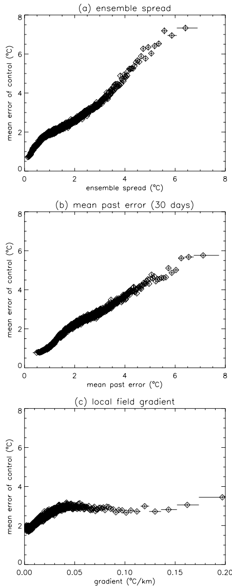
Fig. 5. Plots of the mean forecast error, |\text{verification} - \text{control}| , of sets of 1000 forecasts with similar values of the three predictors of forecast error: (a) ensemble spread, (b) average error of the 30 most recent daily forecasts for which verifications would be available and (c) local field gradient. The horizontal bars represent the ranges of the values of these predictors for each of the 1000 forecasts used to calculate each mean error (for lower values of the predictors these ranges are too small to yield visible bars). The vertical bars represent the standard error in the estimate of the mean forecast error. The forecasts used were the ECMWF ensemble forecasts of the 2-m temperature over North America at a lead time of 96 h initialized on each of the 322 days starting with 4 February 2004.
