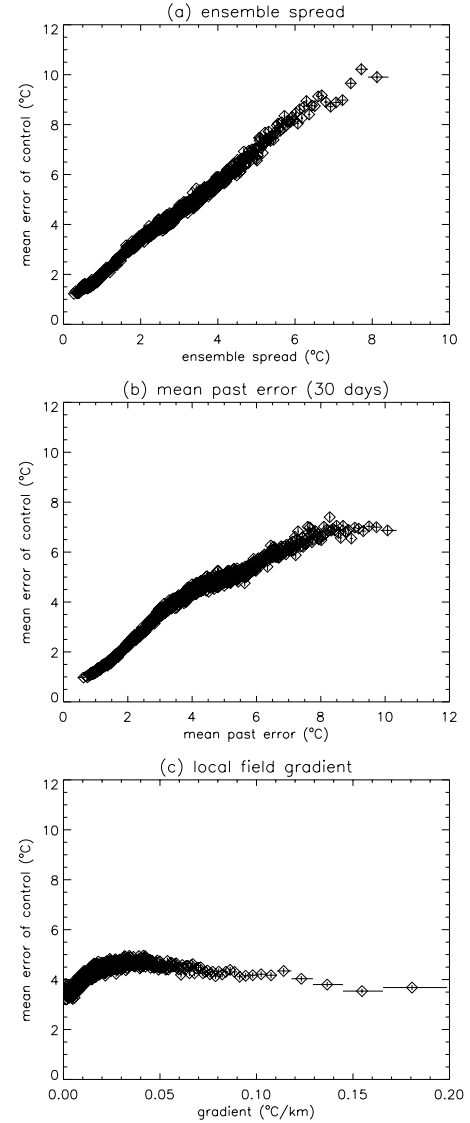
Fig. 7. As Fig. 5 but for a lead time of 240 h. First forecast was issued on 10 February 2004.
