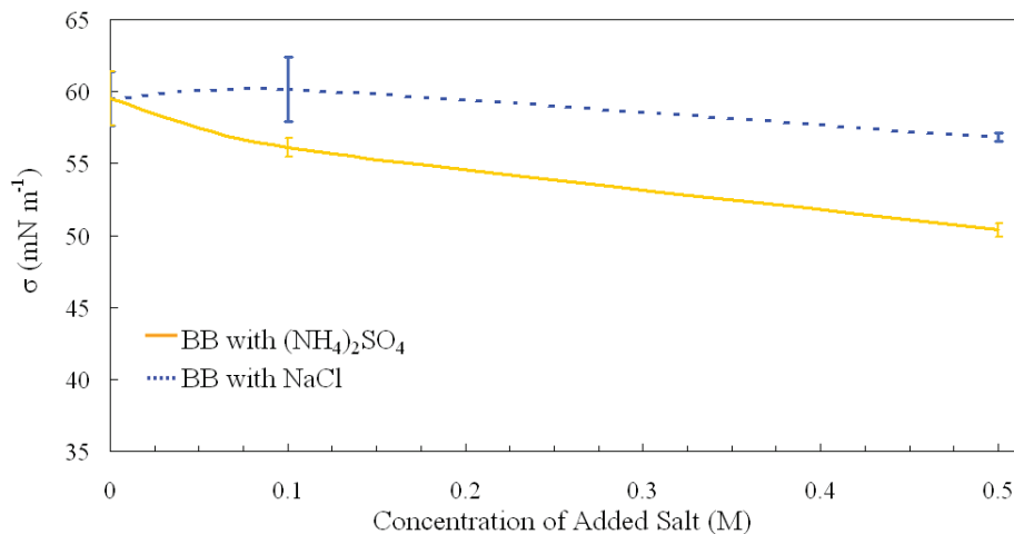
Fig. 5. Surface Tension of BB sample with the addition of (NH 4 ) 2 SO 4 and NaCl. WSOC concentration is constant at 850 mg L -1 ).
