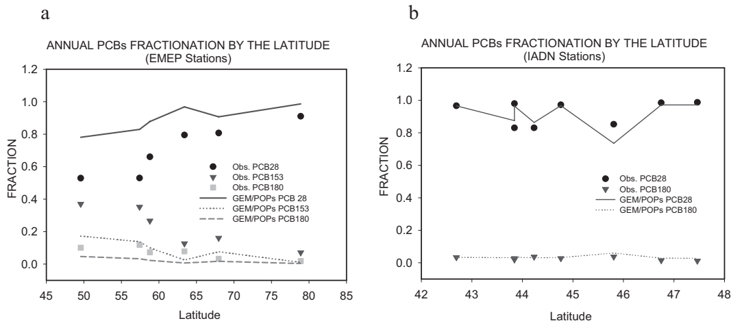
Fig. 4. Comparisons of PCB fractionations at (a) Europe and (b) North American stations.
