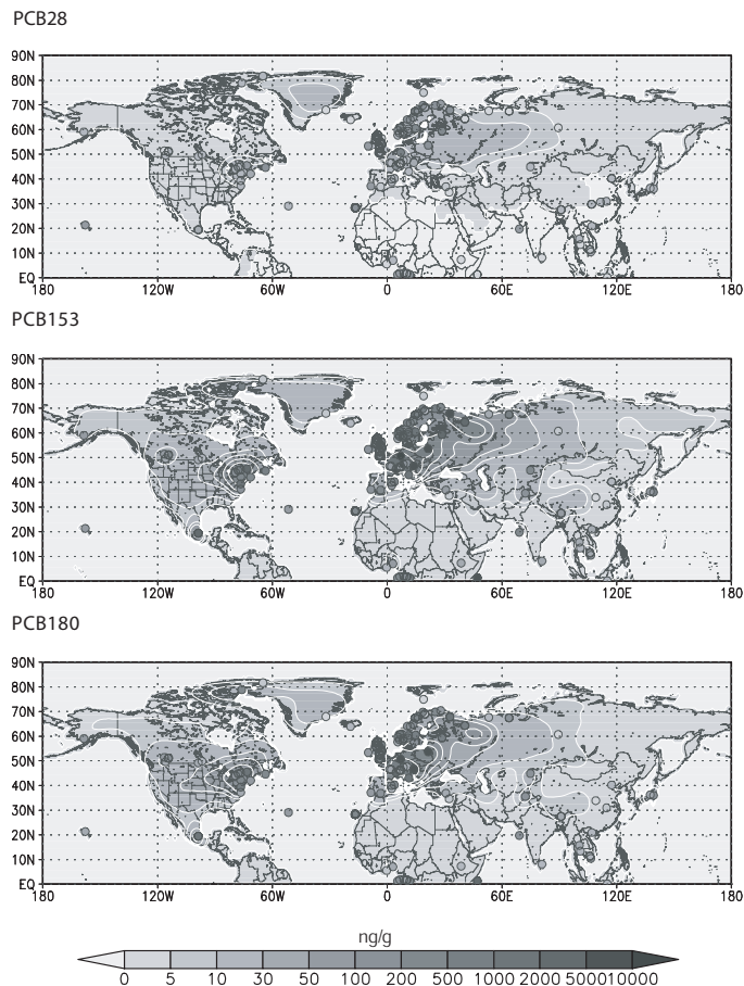
Fig. 1. Assimilated three PCB soil concentrations from MSC-East hemispheric POP model outputs, soil concentrations (Meijer et al., 2003) and data from China (Table 1). The observed locations and concentrations are expressed as a lined circle filled with the same color scale as the contour plots.
