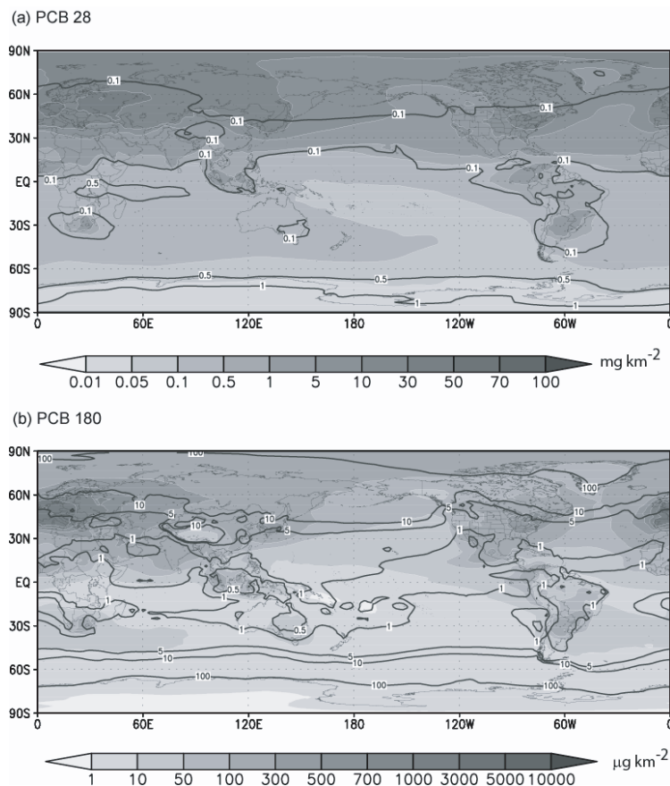
Fig. 5. Column loadings of the total atmospheric PCB28 and PCB180 (filled contours) and ratios of particulate to gaseous PCB28 and PCB180 (contour lines) in the atmosphere for spring of 2000.
