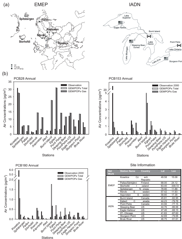
Fig. 2. (a) Geographic locations of EMEP and IADN master stations. (b) Comparisons of observed and simulated annual averaged PCB28, 153 and 180 for 2000.
