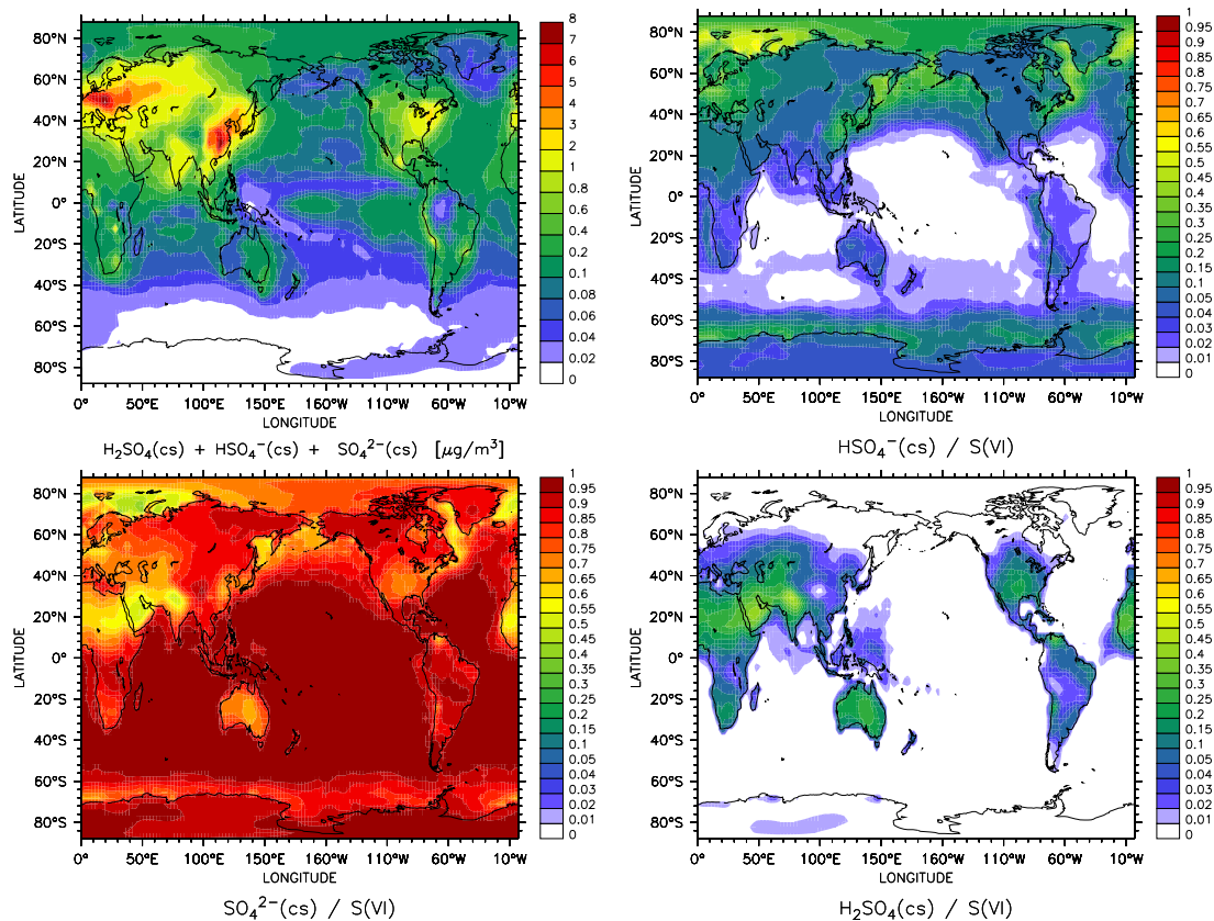
Fig. 4. Upper left: Annual average concentration (in \mu\text{g}/\text{m}^3 ) of sulphur VI (S(VI)) in the lowest model layer. The other panels show the fractions of the individual S(VI) compounds ( \text{HSO}_4^- , \text{SO}_4^{2-} and \text{H}_2\text{SO}_4 ).
