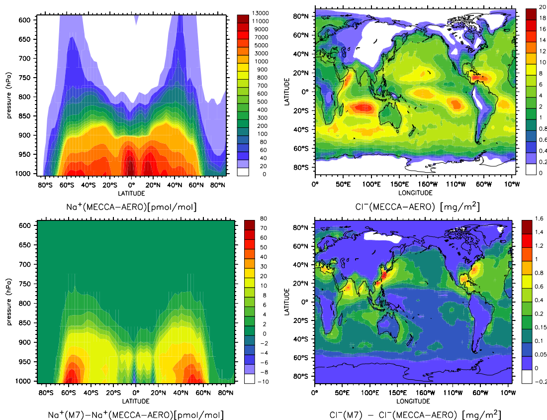
Fig. 3. Left top: Annual average \text{Na}^+ mixing ratios (in \text{pmol/mol} ) calculated by MECCA-AERO for 180^\circ\text{West} . Left bottom: Annual average difference of \text{Na}^+ mixing ratios (in \text{pmol/mol} ) calculated by M7 and MECCA-AERO for 180^\circ\text{West} . Right top: Annual average burden (in \text{mg/m}^2 ) of \text{Cl}^- calculated by MECCA-AERO. Right bottom: Difference of annual average burdens (in \text{mg/m}^2 ) of \text{Cl}^- calculated by M7 and MECCA-AERO, respectively.
