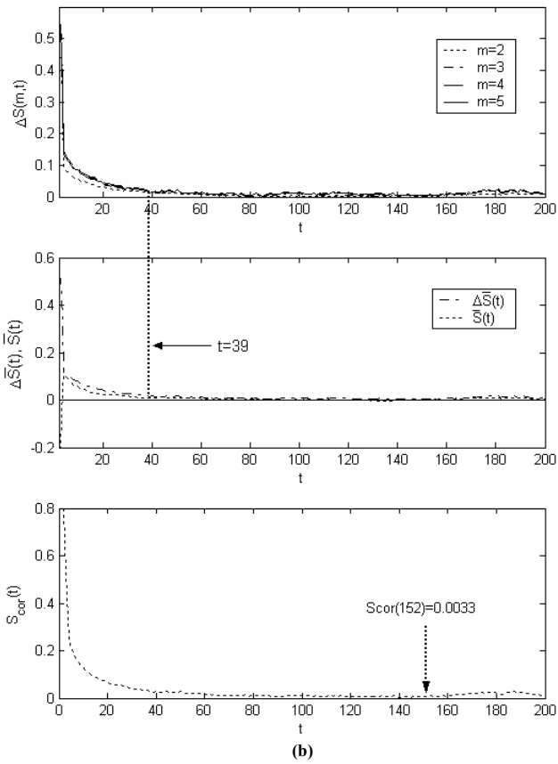
Fig. 2. Estimations of \tau_d and \tau_w for the St. Marys River, Florida, USA: (a) S(m, r, t) and (b) \Delta S(m, t) , \Delta \bar{S}(t) , \bar{S}(t) , and S_{cor}(t) .
