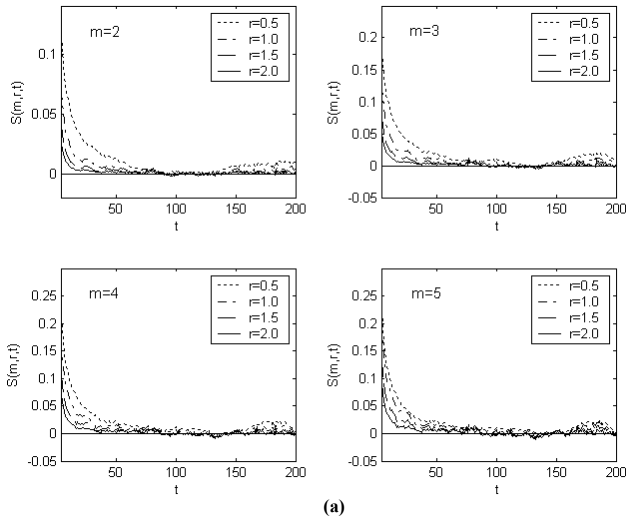
Fig. 3. Estimation of the correlation dimension using the delay time \tau_d for the daily flows of the St. Marys River, Florida, USA: (a) correlation integral and its linear regions (shown as full lines) and (b) slopes (correlation dimension) vs. embedding dimension.
