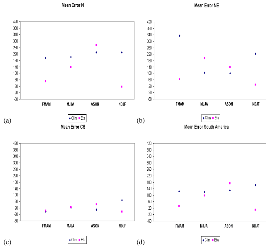
Fig. 16. Mean precipitation forecast errors (squares) and climatology errors (diamonds) (mm) in the regions: (a) Amazon, (b) Northeast, (c) Center-South and (d) whole South America.
