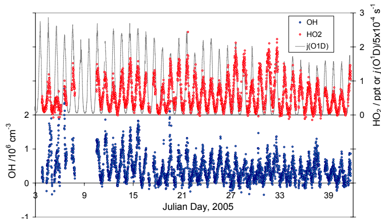
Fig. 2. Time series of OH (molecule \text{cm}^{-3} ; blue) and HO 2 (ppt, red, upper panel) data for the campaign, together with j(\text{O}^1\text{D}) ( \text{s}^{-1} ; black line, upper panel).
