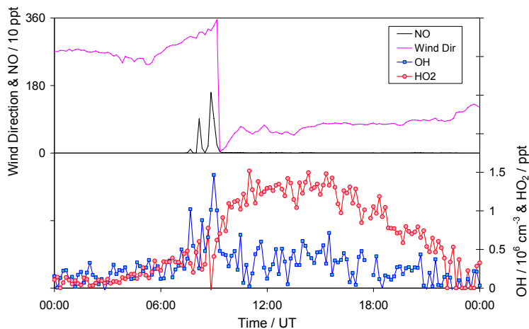
Fig. 3. HO x perturbation due to base pollution event of 30th January. Time series of OH (red circles, 10 6 molecule cm -3 ) and HO 2 (blue circles, ppt) (lower panel), together with NO (black line, ppt/10) and local wind direction (pink line) (upper panel).
