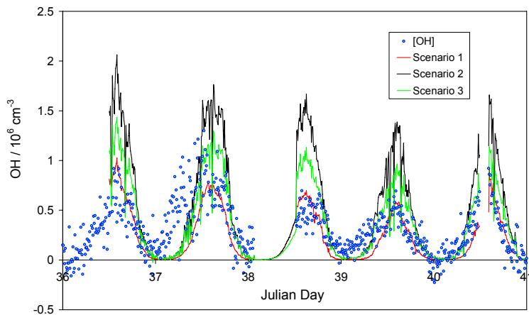
Fig. 7. Measured OH concentrations for 6th–10th February 2005, days 36–40, together with calculated steady-state levels; see text for details.
