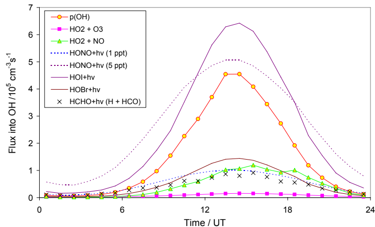
Fig. 6. Calculated mean diurnal variation of principal OH production mechanisms over the measurement period; see text for details.
