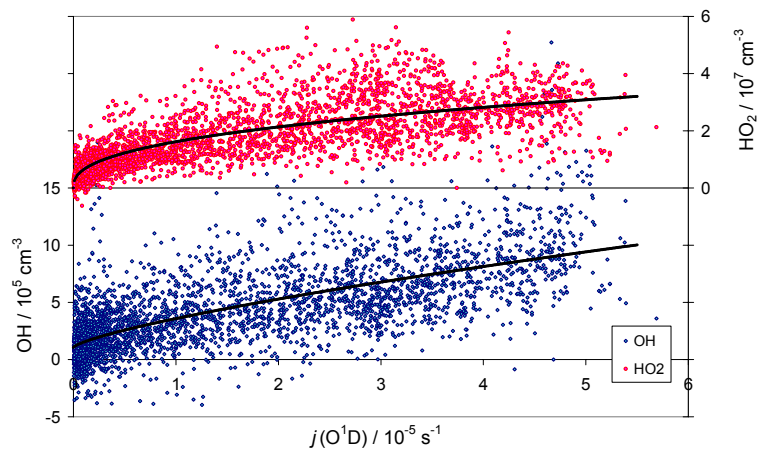
Fig. 5. Variation of clean-air sector OH and HO 2 data with j(O^1D) , together with fits to Eq. (3).
