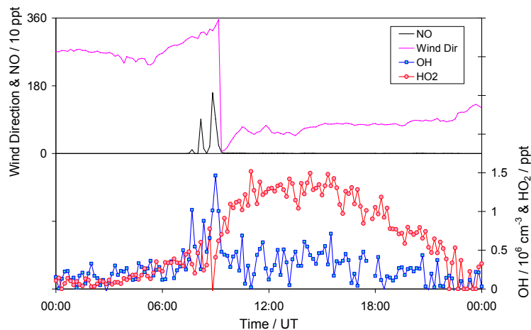
Fig. 3. HO x perturbation due to base pollution event of 30th January. Time series of OH (red circles, 10 6 molecule cm -3 ) and HO 2 (blue circles, ppt) (lower panel), together with NO (black line, ppt/10) and local wind direction (pink line) (upper panel).
