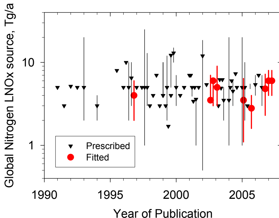
Fig. 28. Global annual nitrogen mass LNO x source as prescribed or fitted to data in global atmospheric model studies versus year of publication, as listed in Table 24. Triangles with vertical bars denote estimated values and expected uncertainty ranges. Thick red dots with error bars denote model fit LNO x results and the derived uncertainty ranges (Levy et al., 1996; Martin et al., 2002b, 2007; Tie et al., 2002; Staudt et al., 2003; Boersma et al., 2005; Müller and Stavrou, 2005; Schumann et al., 2006; Sauvage et al., 2007).
