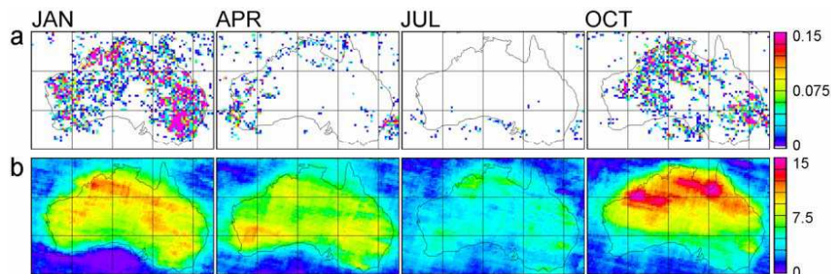
Fig. 16. Monthly mean LIS flash counts (upper row, flashes per day and km) and GOME tropospheric NO 2 column (lower row, 10^{14} molecules \text{cm}^{-2} ; corrected for air mass factors) in Australia for several months in 1999 as discussed in Beirle et al. (2004b); figure from Beirle (2004), with kind permission of Elsevier.
