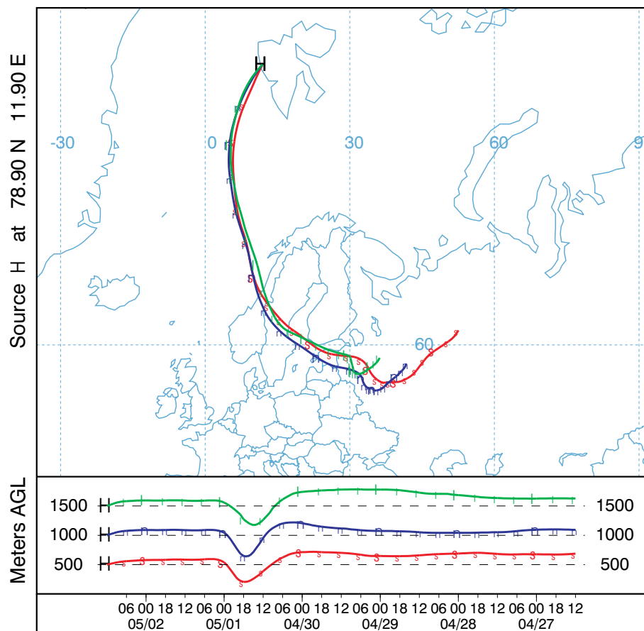
Fig. 1. 5 days back trajectories at 500 m, 1000 m and 1500 m a.g.l. for the air mass arriving in Ny-Ålesund on 2 May 2006 (12:00 UTC) as computed by the HYSPLIT model. Data source: NOAA-ARL.
