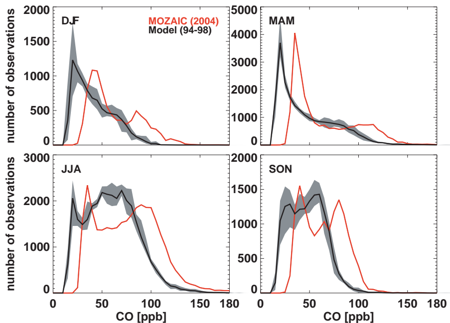
Fig. 3. A comparison of the MOZAIC (red) and model (black) CO for flights between East Asia and Europe. The gray shaded area shows the range of the model during 1994–1998. The aircraft data are from 2004.
